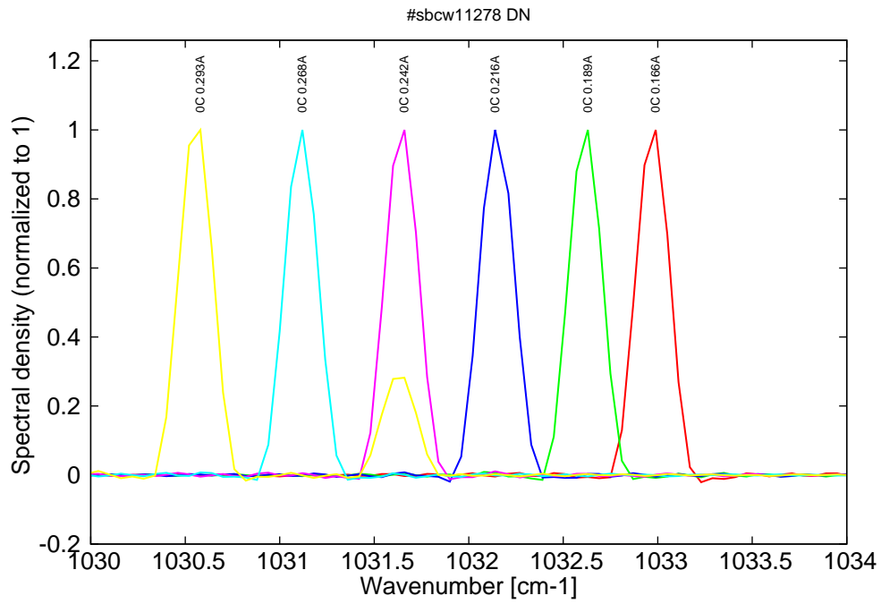
Figure 10: spectra at 0C for various DC currents (monomode up to 0.265A, then becomes bimode)
