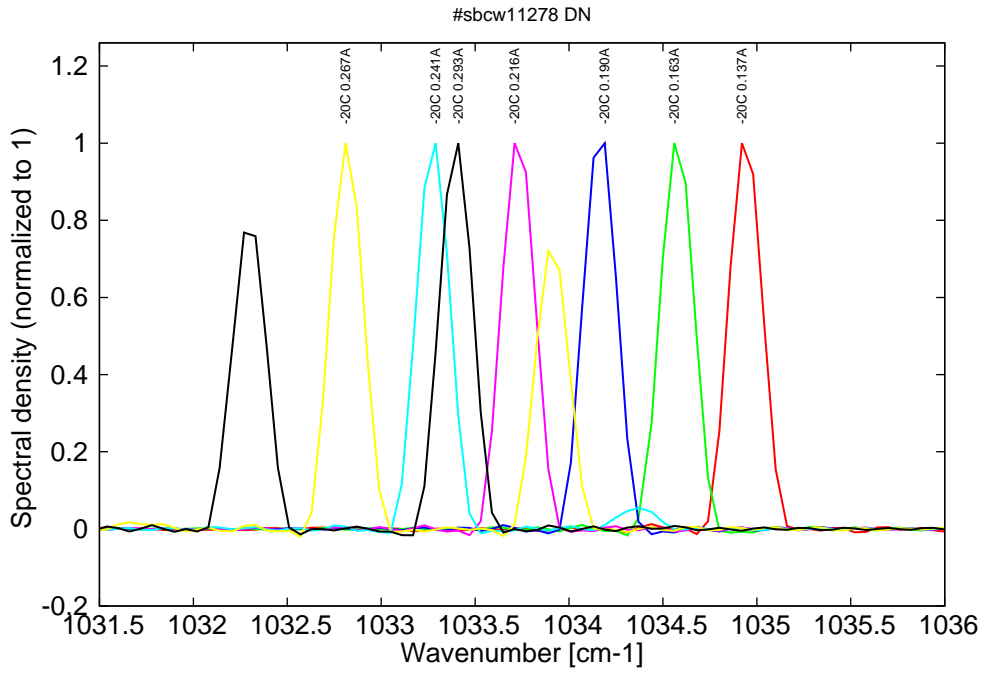
Figure 6: spectra at -20C for various DC currents (monomode up to 0.215A, then becomes bimode)
