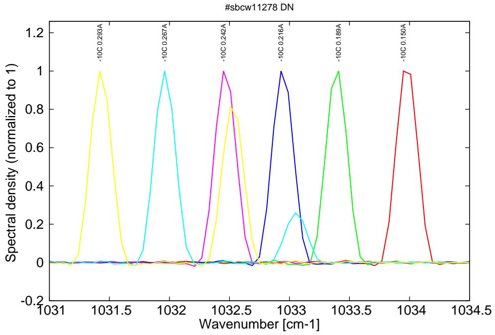
Figure 8: spectra at -10C for various DC currents (monomode up to 0.240A, then becomes bimode)
