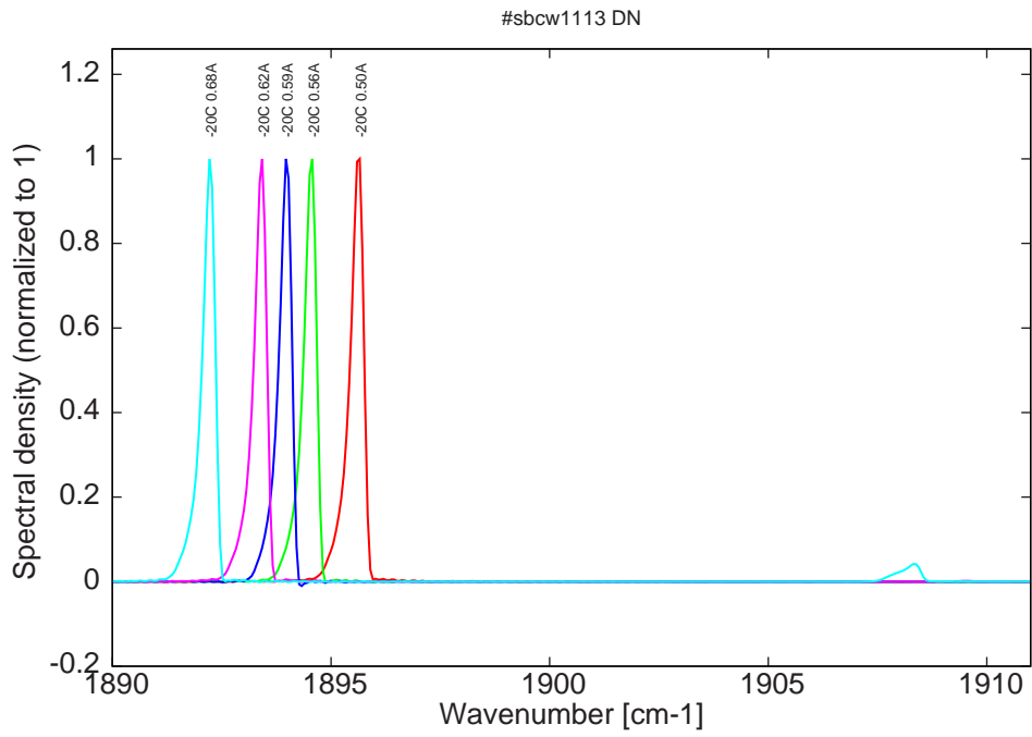
Figure 8: spectra at -20C for various DC currents (monomode up to 0.59A)
