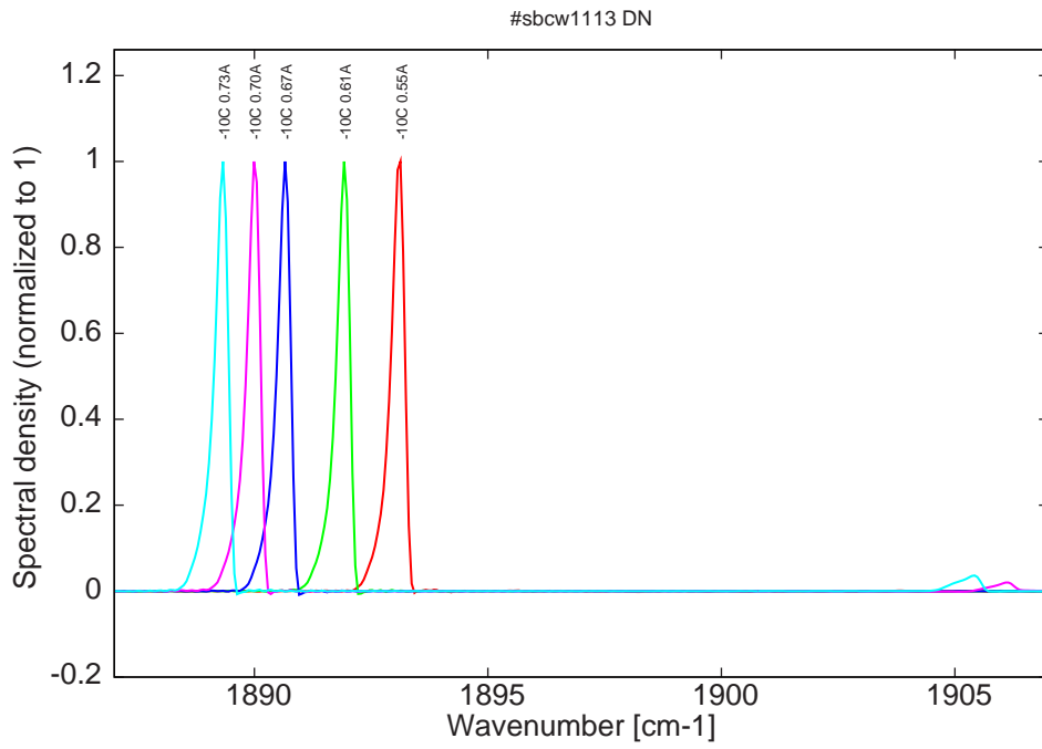
Figure 10: spectra at -10C for various DC currents (monomode up to 0.67A)
