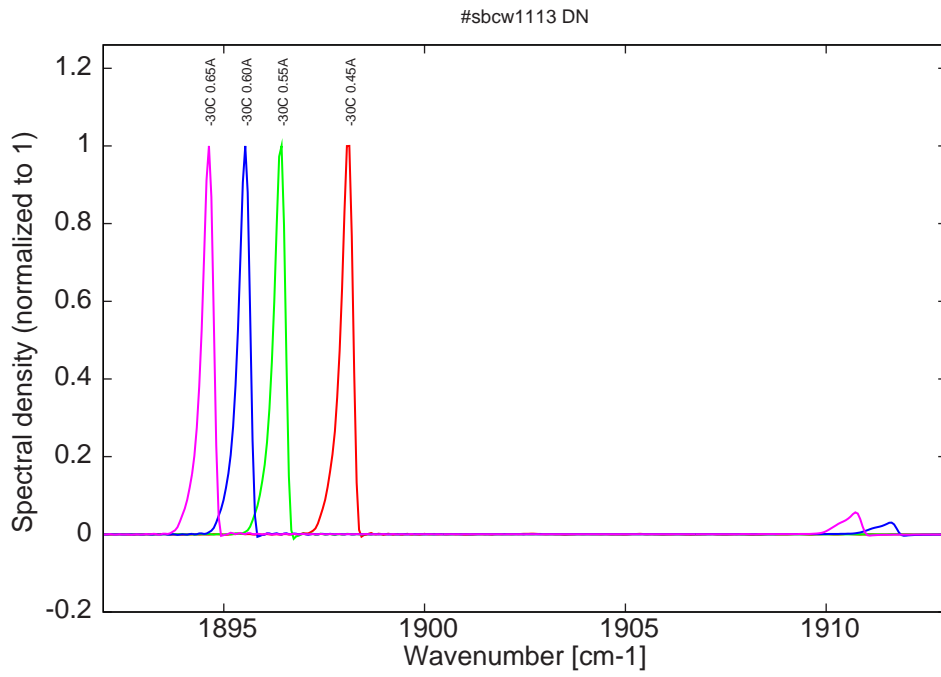
Figure 6: spectra at -30C for various DC currents (monomode up to 0.55A)
