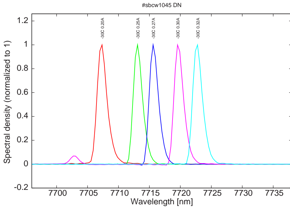
Figure 6: spectra at -30C for various DC currents (become monomode again at 0.32A)
