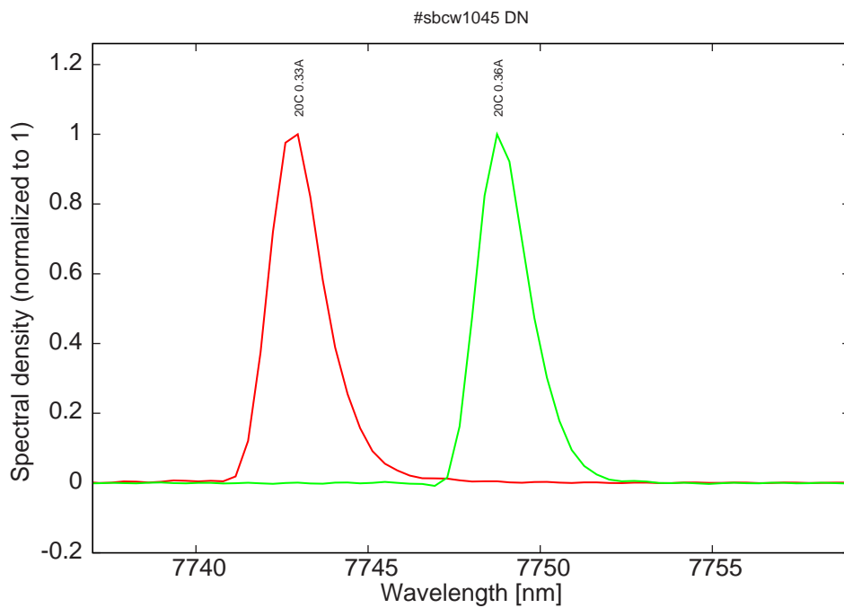
Figure 13: spectra at 20C for various DC currents (same mode compared to spectra at 10C at high current)
