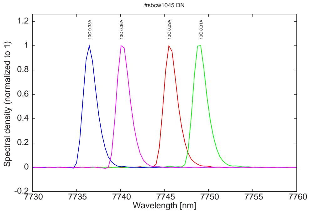
Figure 12: spectra at 10C for various DC currents (all monomode, but with mode jumping for current higher than 0.33A)
