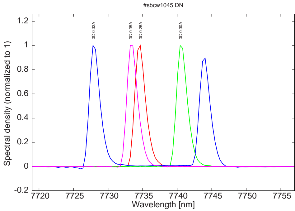
Figure 10: spectra at 0C for various DC currents (become monomode again at 0.35A, but with mode jumping)
