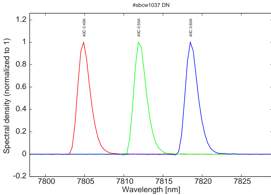
Figure 15: spectra at 40C for various DC currents
