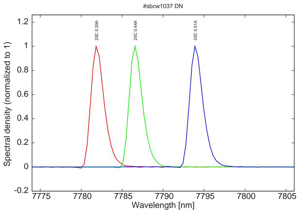
Figure 13: spectra at 20C for various DC currents (monomode range)
