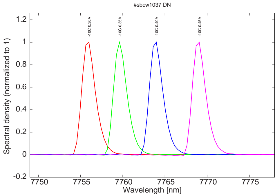
Figure 10: spectra at -10C for various DC currents (monomode range)
