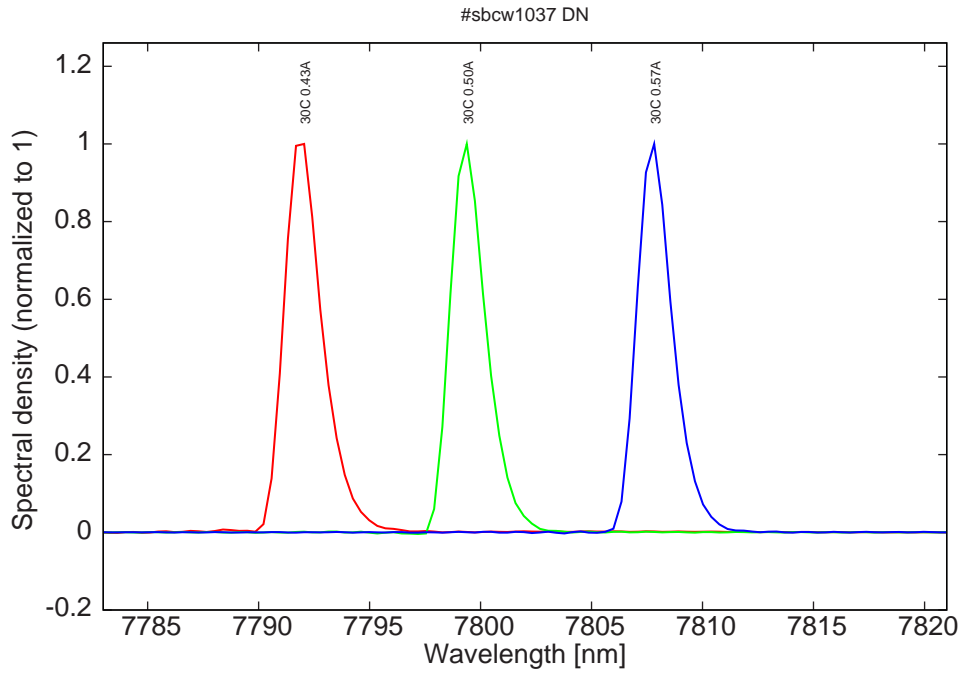
Figure 14: spectra at 30C for various DC currents (monomode range)
