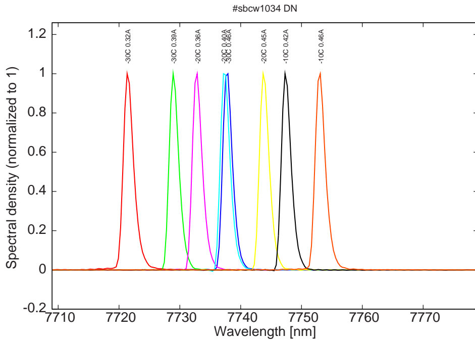
Figure 5: spectra at -30C, -20C and -10C for various DC currents
