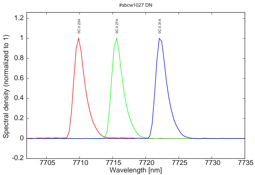
Figure 8: spectra at 0C for various DC currents
