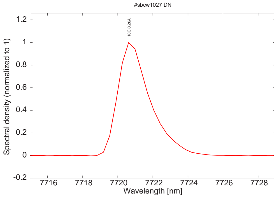
Figure 9: monomode spectrum at 10C and 0.26A
