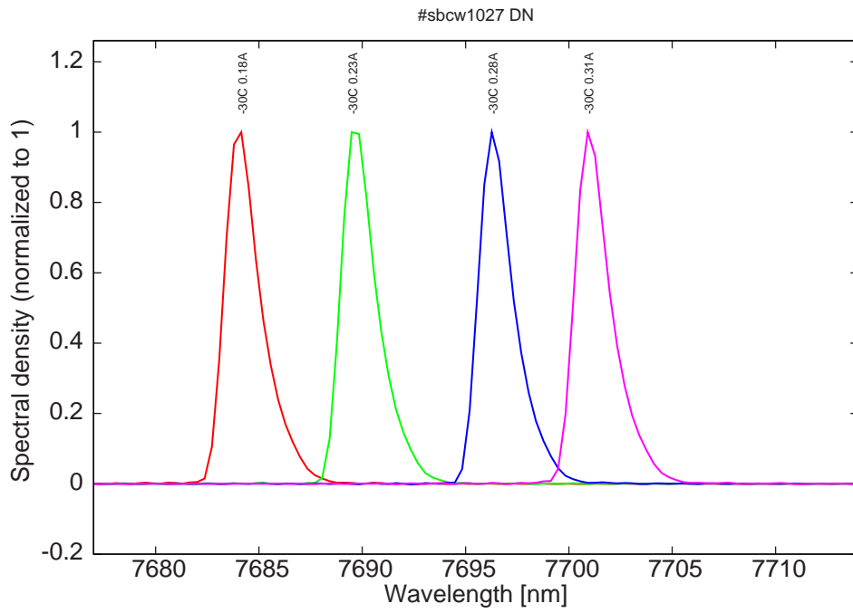
Figure 5: spectra at -30C for various DC currents
