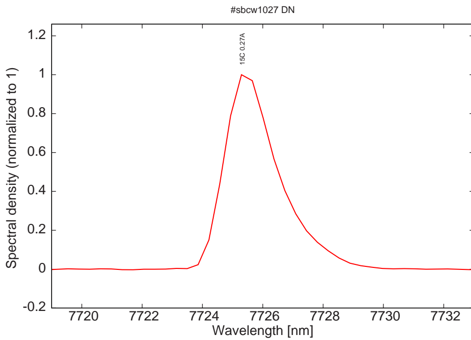
Figure 10: monomode spectrum at 15C and 0.27A
