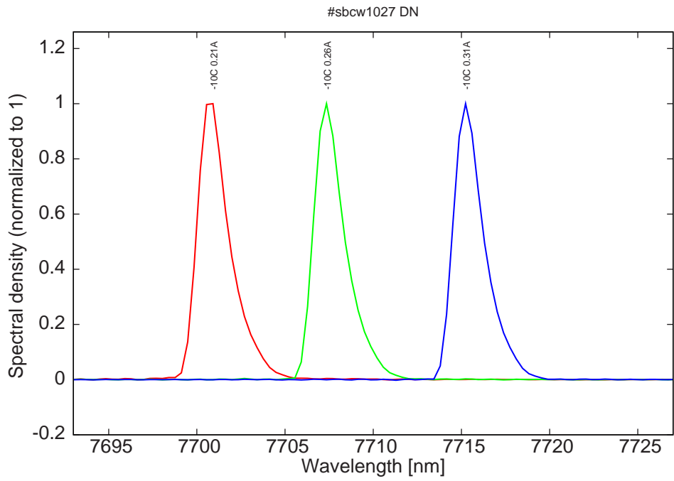
Figure 7: spectra at -10C for various DC currents
