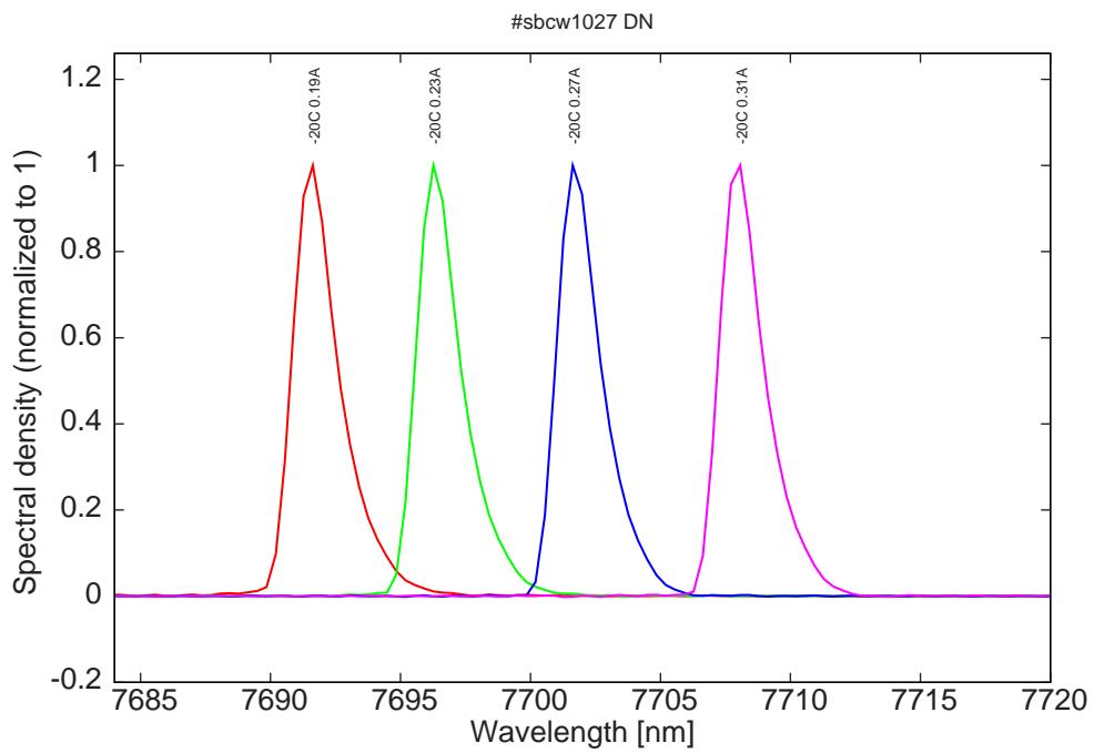
Figure 6: spectra at -20C for various DC currents
