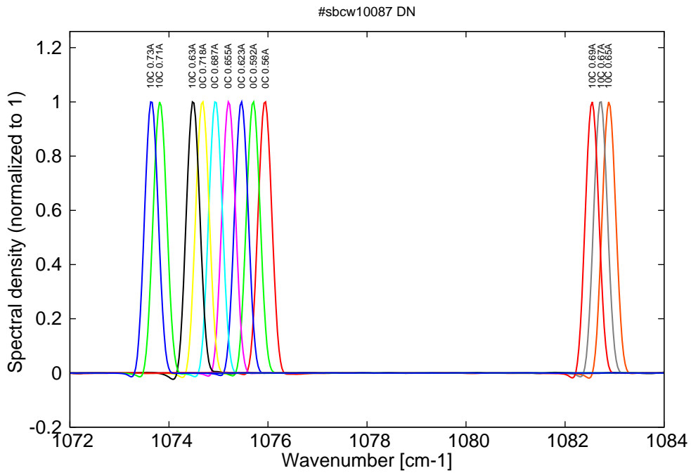
Figure 3: spectra at 0C and 10C in continuous-wave operation (front resistor current I_F = 0A and back resistor current I_B = 0A )
