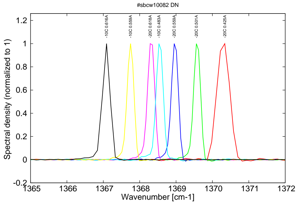
Figure 5: spectra at -20C and -10C for various DC currents (monomode on mode 1)
