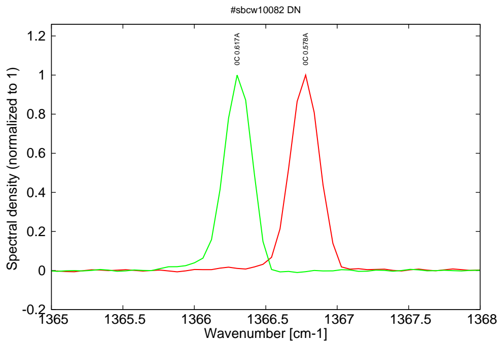
Figure 6: spectra at 0C for various DC currents (monomode on mode 2)
