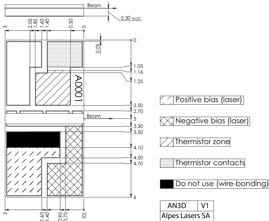
Figure 1: Support mounting for #sbcw10082 DN (please note that AlN submount numbering is P0251)
