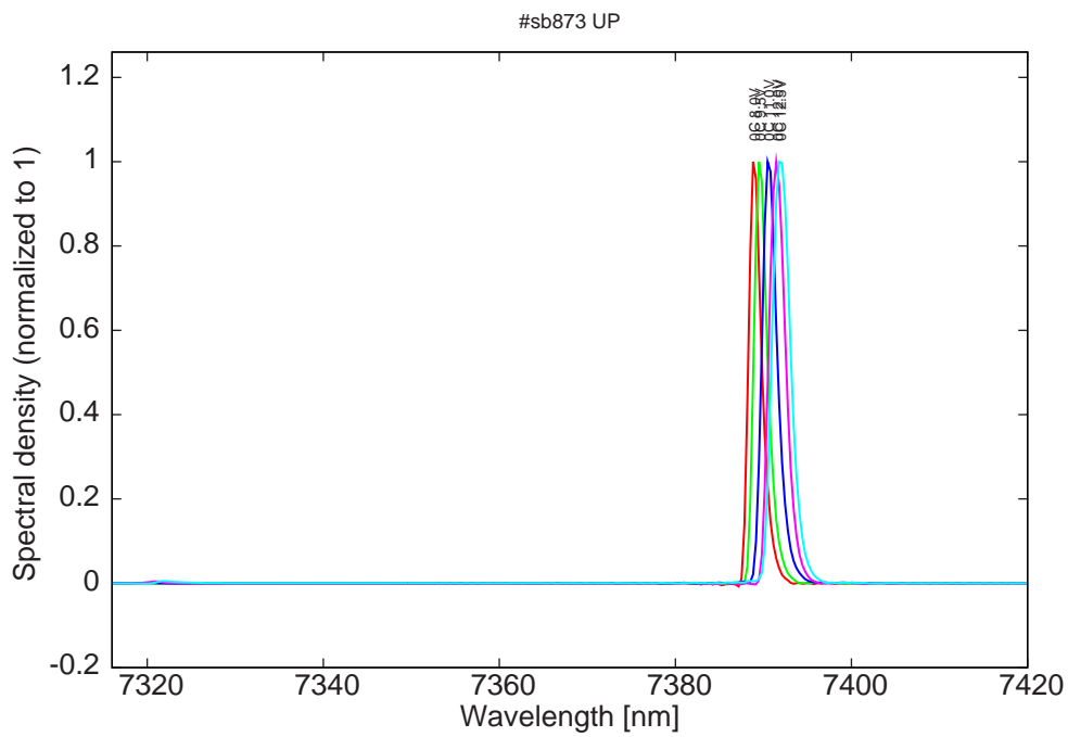
Figure 12: spectra at 0C for various LDD voltages (small mode around 7322nm for high voltage on LDD)
