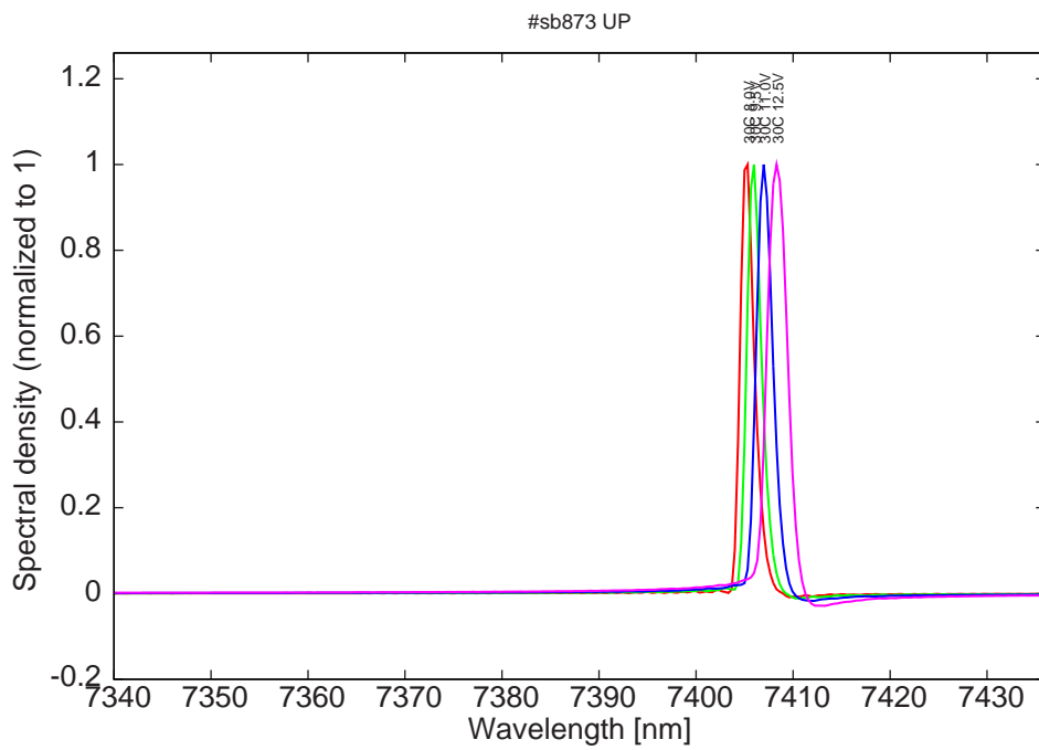
Figure 16: spectra at 30C for various LDD voltages (small mode around 7342nm at 12.5V on LDD)
