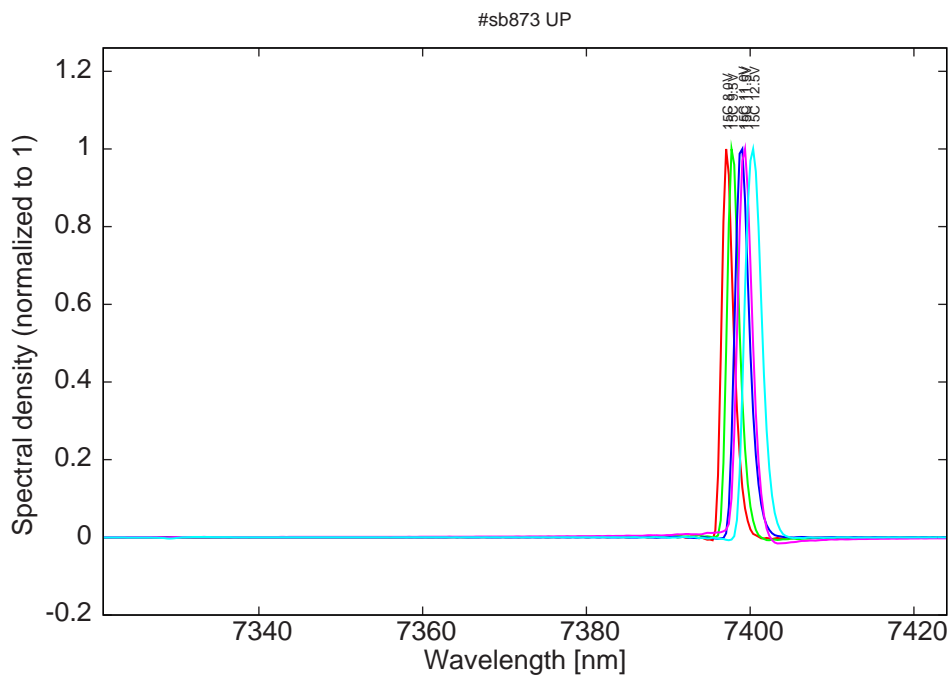
Figure 14: spectra at 15C for various LDD voltages (small mode around 7328nm for high voltage on LDD)
