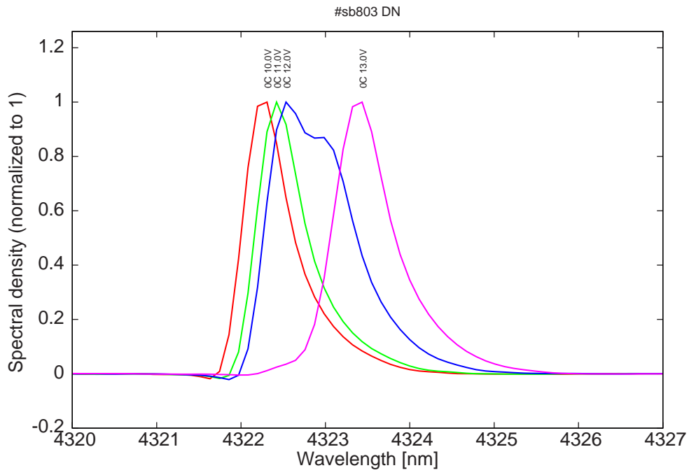
Figure 9: spectra at 0C for various LDD voltages (absorption in the air at 4323nm)
