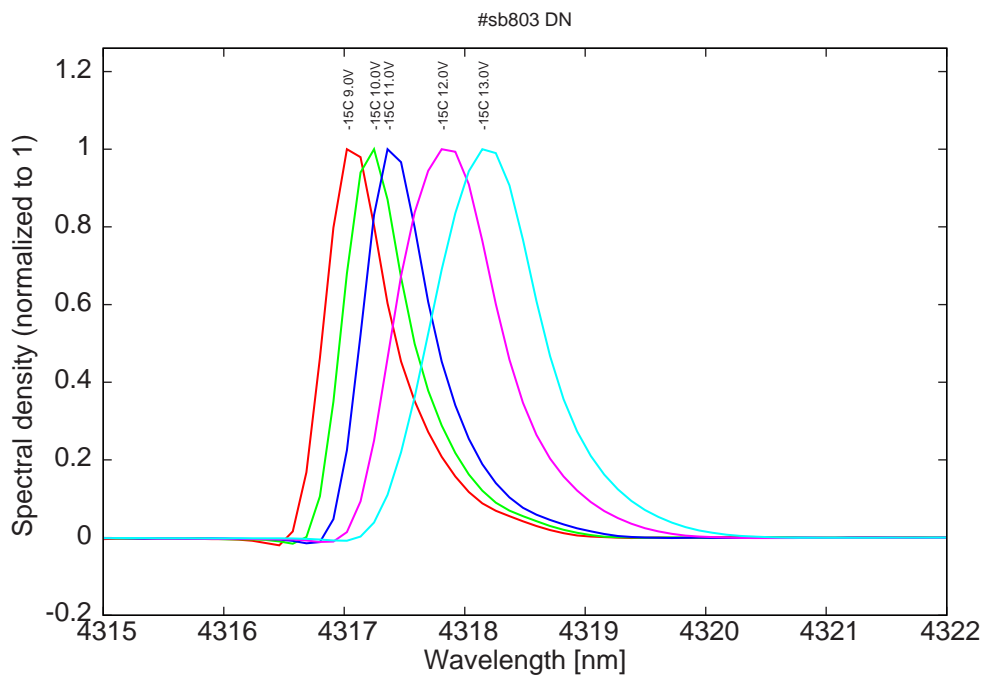
Figure 8: spectra at -15C for various LDD voltages (absorption in the air at 4317.5nm)
