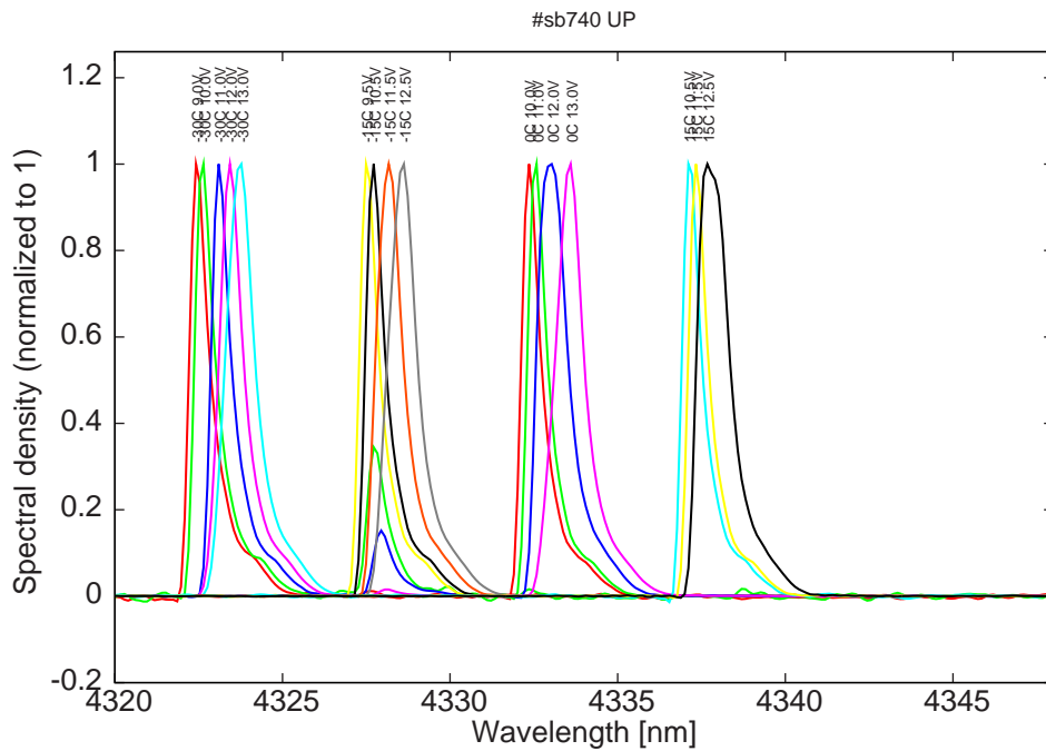
Figure 8: spectra at -30C, -15C, 0C and 15C at 2% dc for various LDD voltages
