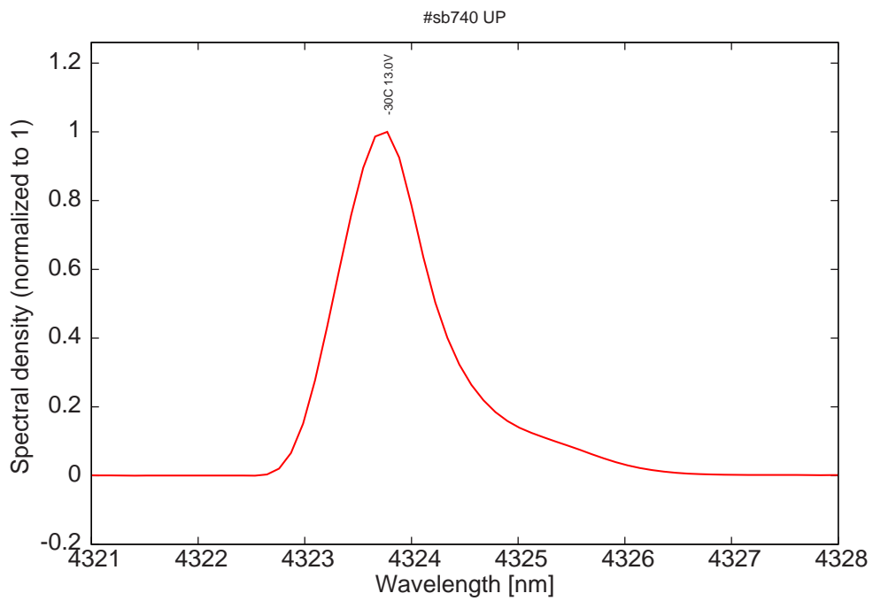
Figure 10: monomode spectrum at -30C and 13V
