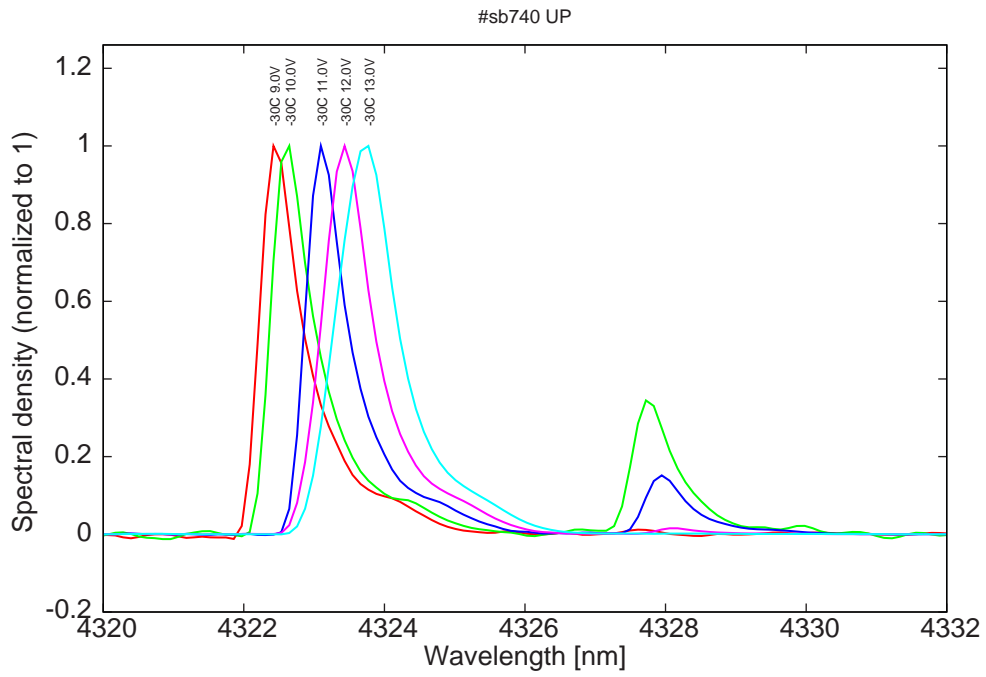
Figure 9: spectra at -30C for various LDD voltages (monomode at high voltage)
