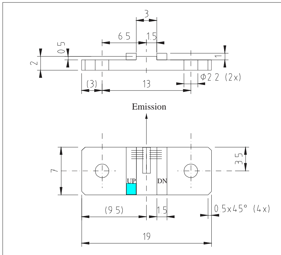
Figure 1: Support mounting for #sb724 UP (please note that the laser is connected to the UP pad drawn in blue)
