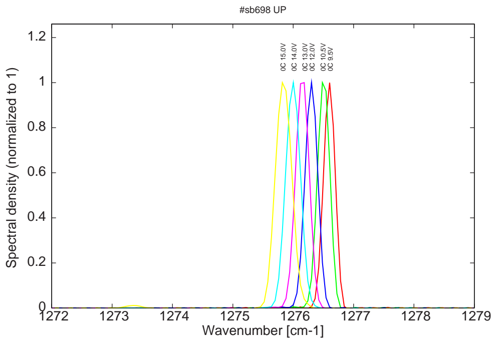
Figure 11: spectra at 0C for various LDD voltages (monomode up to 13V on LDD)
