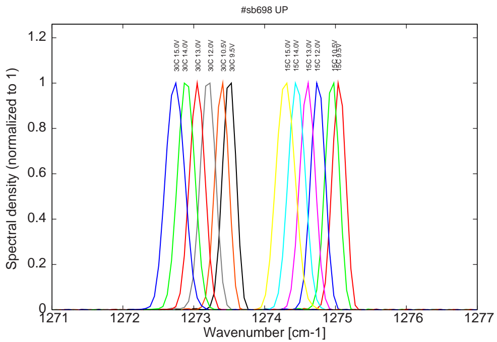
Figure 13: spectra at 15C and 30C for various LDD voltages (all monomode)
