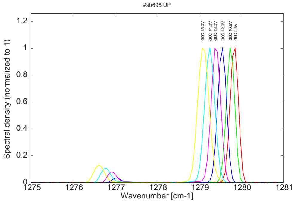
Figure 8: spectra at -30C for various LDD voltages (monomode at threshold)
