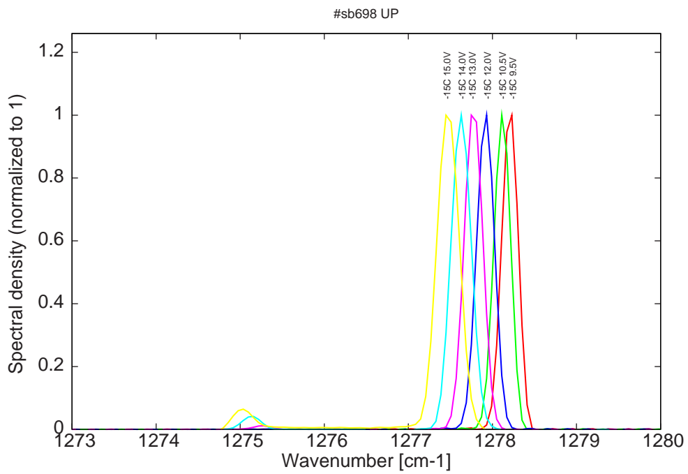
Figure 9: spectra at -15C for various LDD voltages (monomode up to 12V on LDD)
