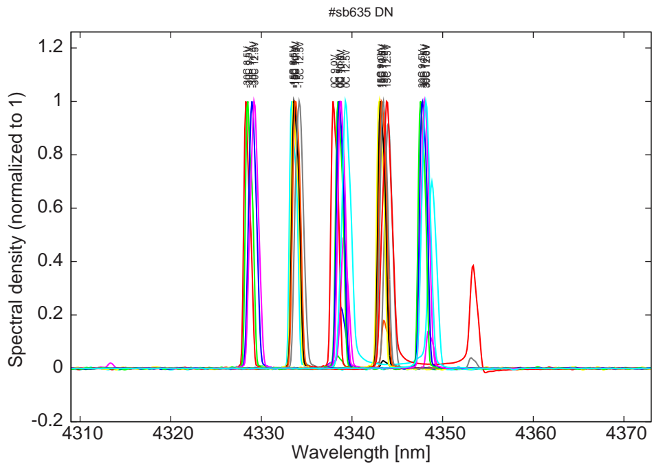
Figure 8: spectra at -30C, -15C, 0C, 15C and 30C at 1% dc (22ns pulses, 2.2 \mu s period) for various LDD voltages
