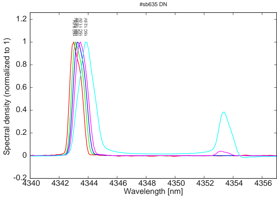
Figure 15: spectra at 15C for various LDD voltages (monomode up to 10.5V)
