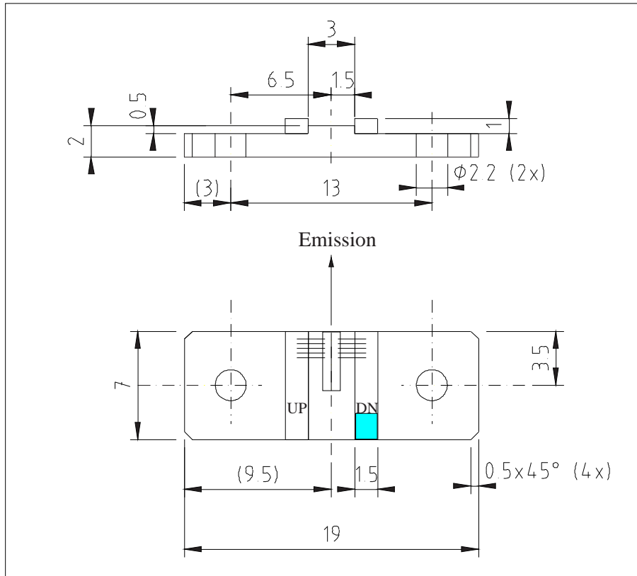
Figure 1: Support mounting for #sb635 DN (please note that the laser is connected to the DN pad drawn in blue)
