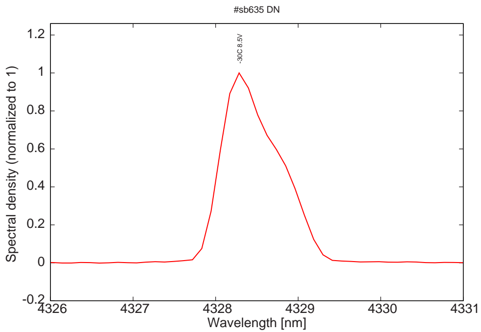
Figure 10: monomode spectrum at -30C and 8.5V on LDD
