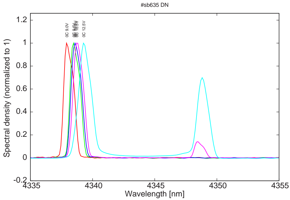
Figure 13: spectra at 0C for various LDD voltages (monomode up to 10V)
