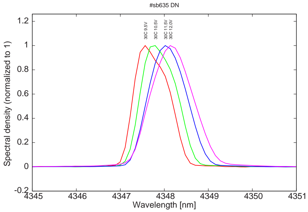
Figure 17: spectra at 30C for various LDD voltages (all monomode)
