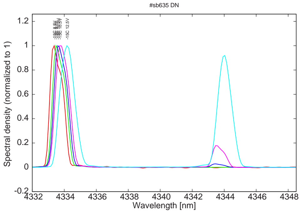
Figure 11: spectra at -15C for various LDD voltages (monomode up to 9.5V)
