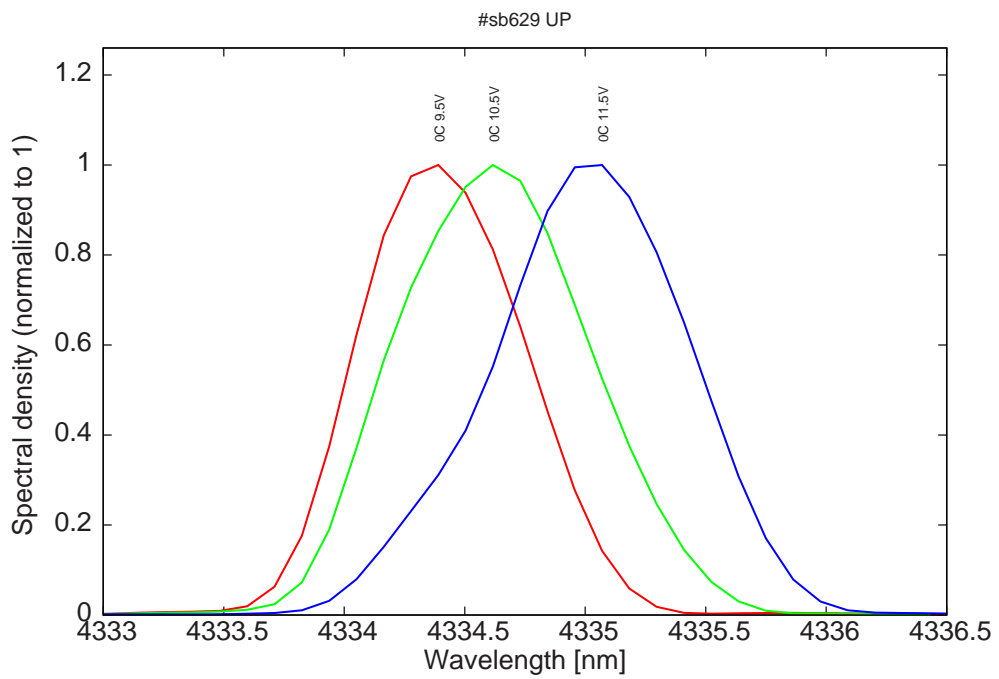
Figure 12: spectra at 0C for various LDD voltages
