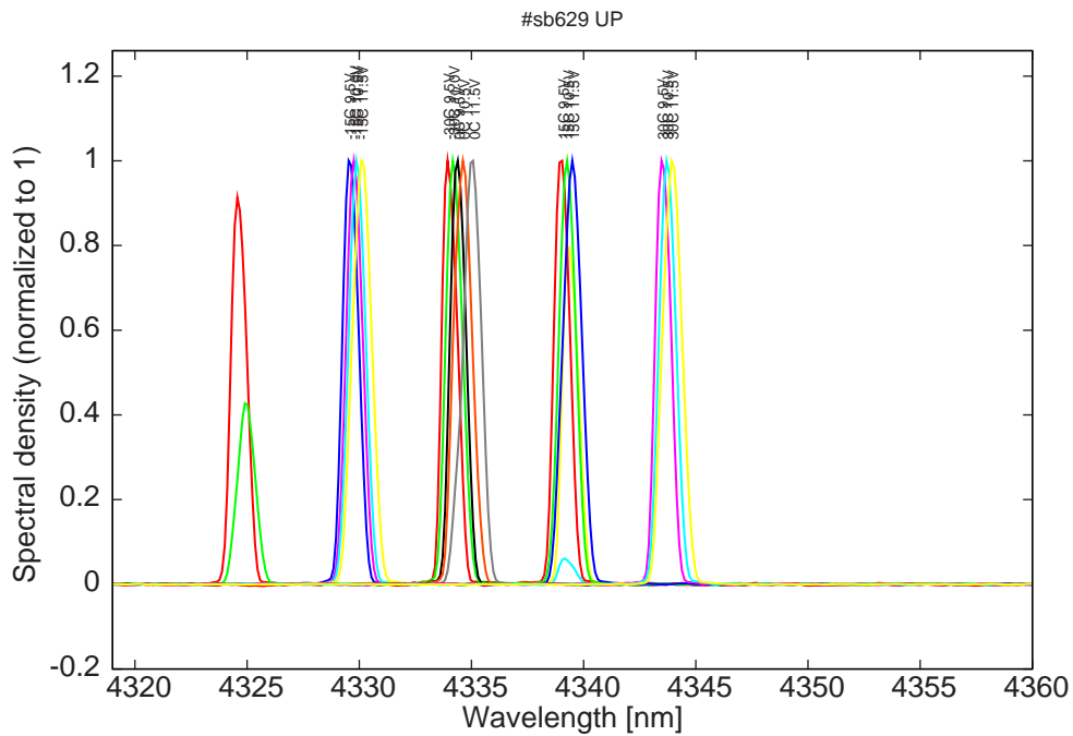
Figure 8: spectra at -30C, -15C, 0C, 15C and 30C at 1% dc (22ns pulses, 2.2 \mu s period) for various LDD voltages
