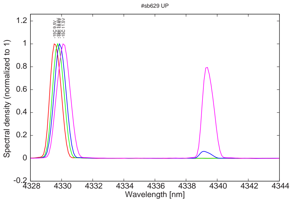
Figure 10: spectra at -15C for various LDD voltages (monomode up to 10V)
