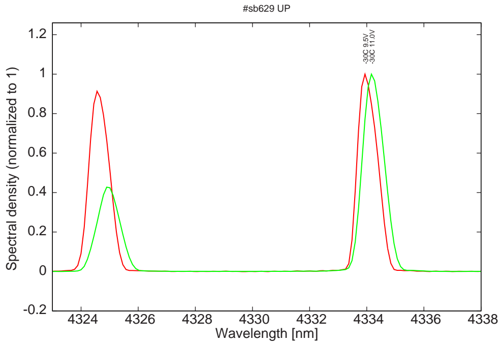
Figure 9: spectra at -30C for various LDD voltages (all bimode)
