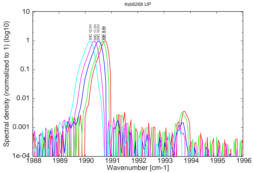
Figure 8: spectra at 30C at 2% duty-cycle (22ns pulses) for various LDD voltages (all bimode)
