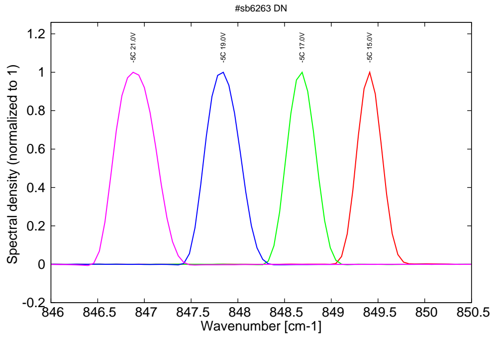
Figure 8: spectra at -5C at 4% duty-cycle
