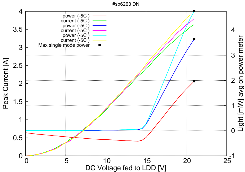
Figure 7: peak current and average power vs LDD voltage at 2% (red), 3% (blue) and 4% (cyan) duty-cycle at -5C (100ns pulses on the laser) (the solid squares indicate the maximum singlemode emitted power)
