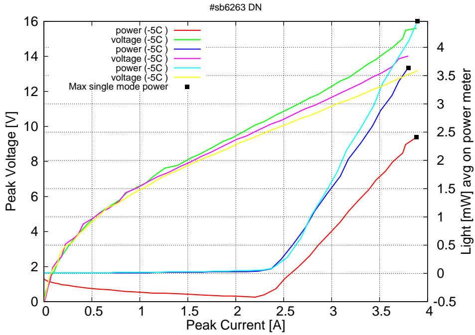
Figure 6: peak voltage and average power vs peak current at 2% (red), 3% (blue) and 4% (cyan) duty-cycle at -5C (100ns pulses on the laser) (the solid squares indicate the maximum singlemode emitted power)
