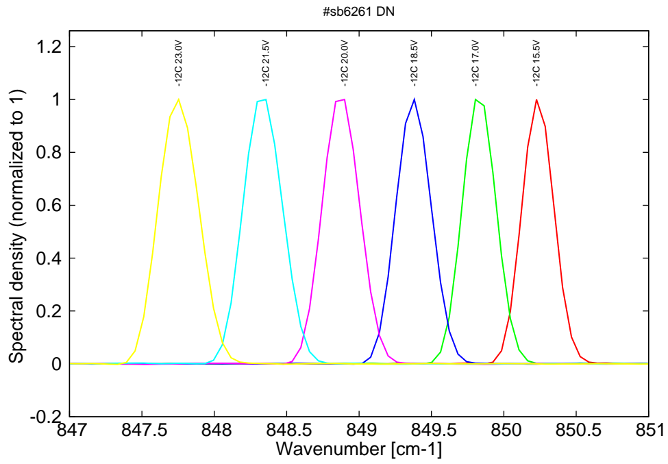
Figure 8: spectra at -12C at 4% duty-cycle
