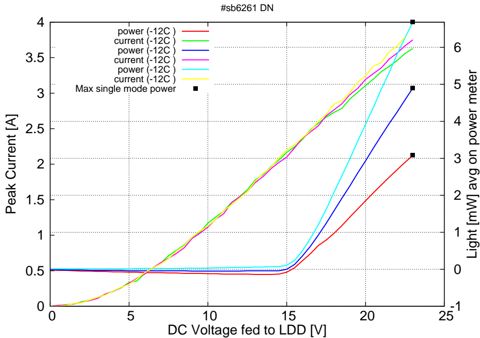
Figure 7: peak current and average power vs LDD voltage at 2% (red), 3% (blue) and 4% (cyan) duty-cycle at -12C (50ns pulses on the laser) (the solid squares indicate the maximum singlemode emitted power)
