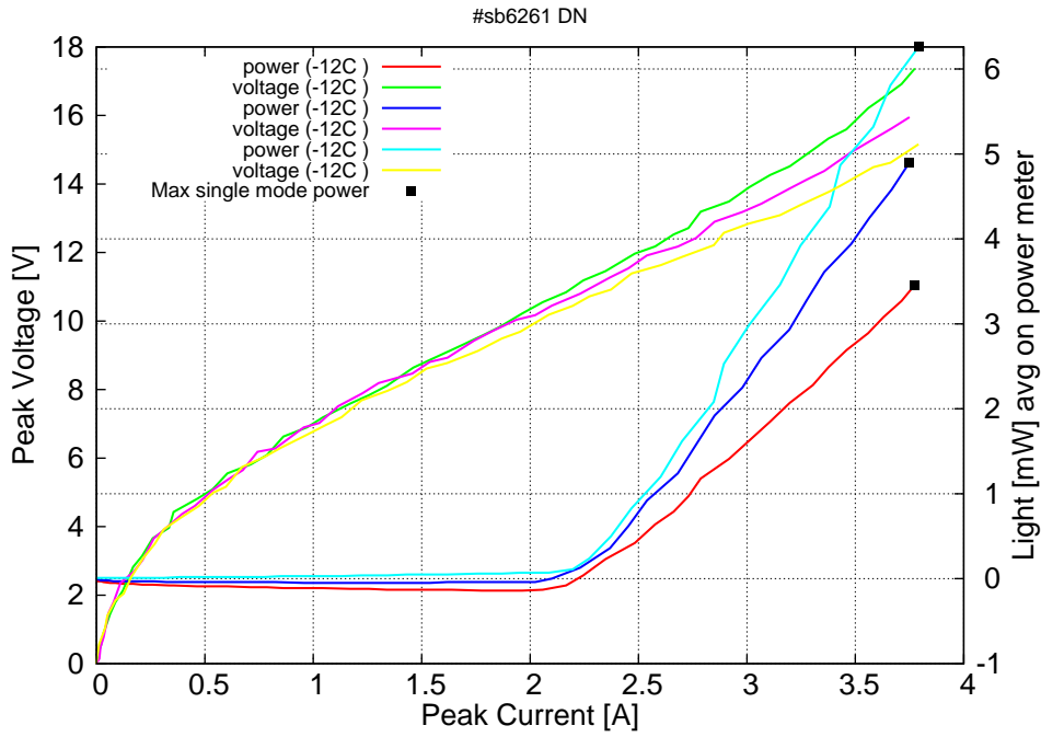
Figure 6: peak voltage and average power vs peak current at 2% (red), 3% (blue) and 4% (cyan) duty-cycle at -12C (50ns pulses on the laser) (the solid squares indicate the maximum singlemode emitted power)
