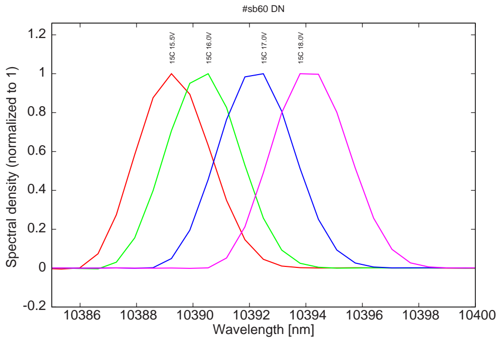
Figure 12: spectra at 15C for various LDD voltages
