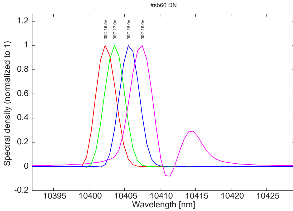
Figure 13: spectra at 30C for various LDD voltages
