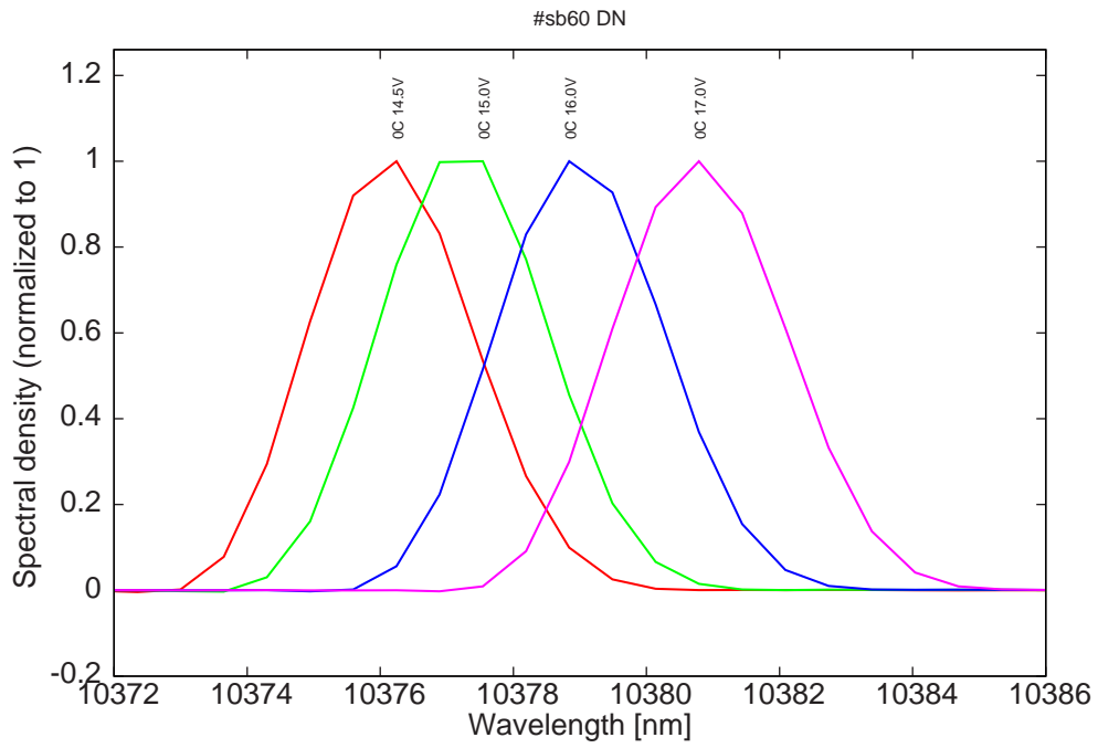
Figure 11: spectra at 0C for various LDD voltages
