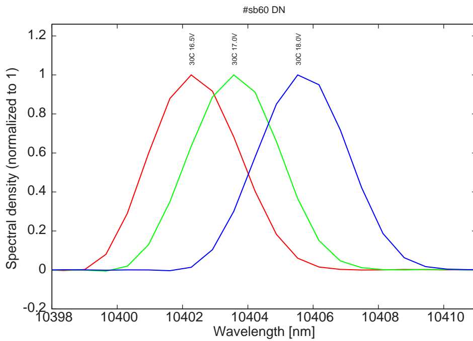
Figure 14: spectra at 30C for various LDD voltages (monomode range)
