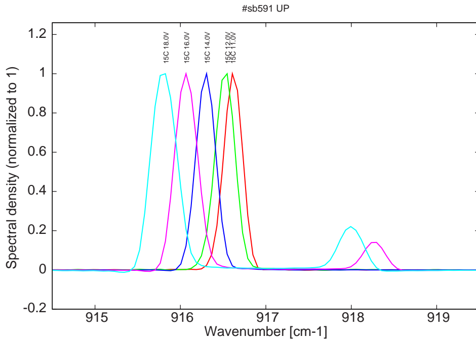
Figure 14: spectra at 15C for various LDD voltages (monomode up to 14V on LDD)
