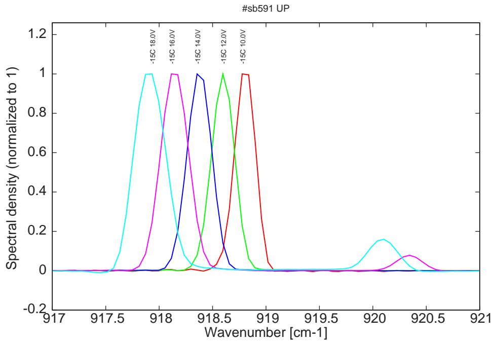
Figure 10: spectra at -15C for various LDD voltages (monomode up to 14V on LDD)
