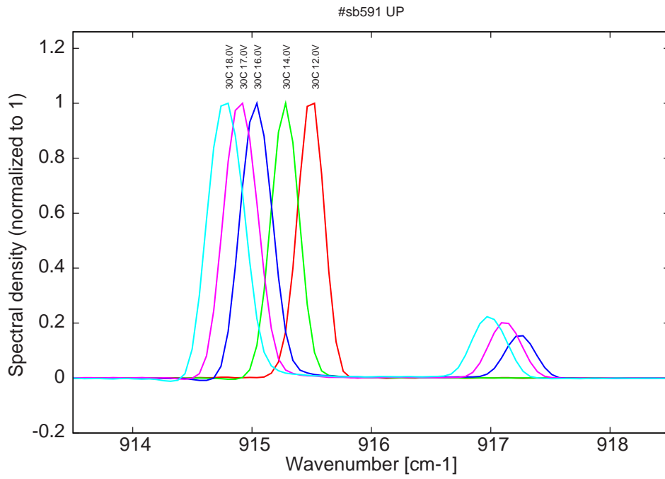
Figure 16: spectra at 30C for various LDD voltages (monomode up to 14V on LDD)
