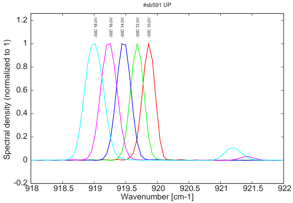
Figure 8: spectra at -30C for various LDD voltages (monomode up to 14V on LDD)
