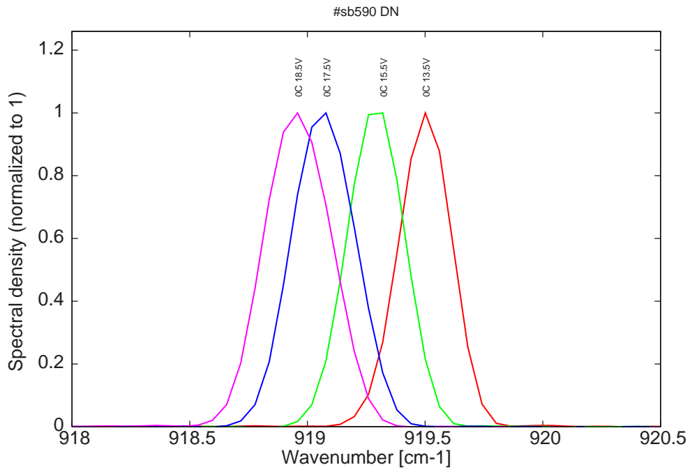
Figure 12: spectra at 0C for various LDD voltages (monomode range)
