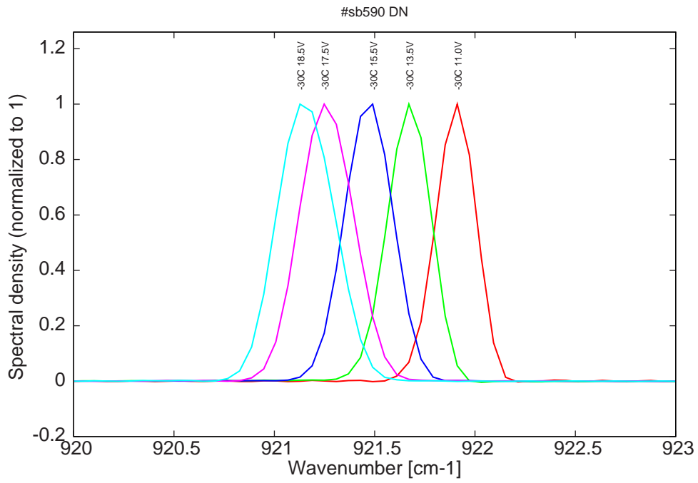
Figure 8: spectra at -30C for various LDD voltages (all monomode)
