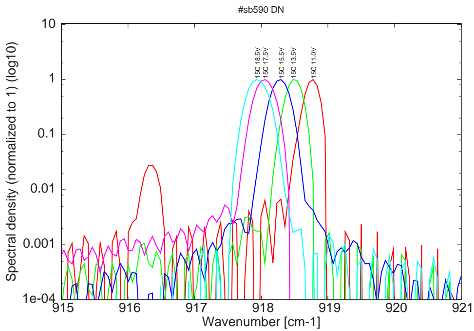
Figure 13: spectra at 15C for various LDD voltages (bimode at threshold)
