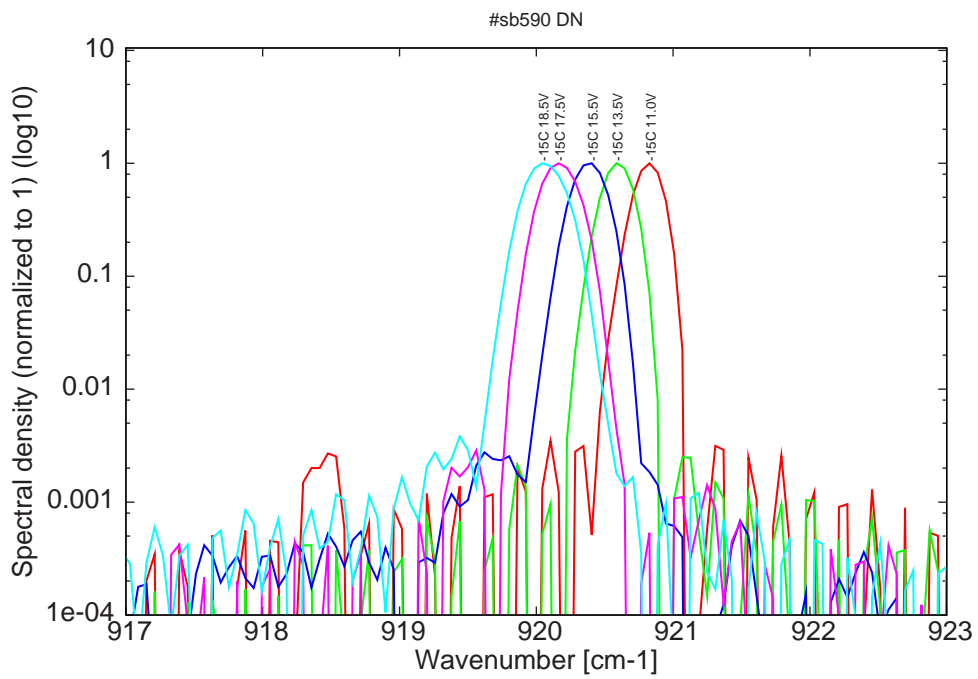
Figure 9: spectra at -15C for various LDD voltages (bimode at threshold)
