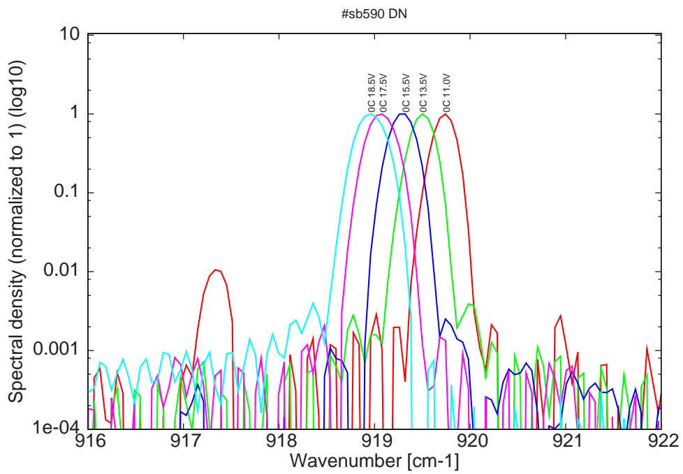
Figure 11: spectra at 0C for various LDD voltages (bimode at threshold)
