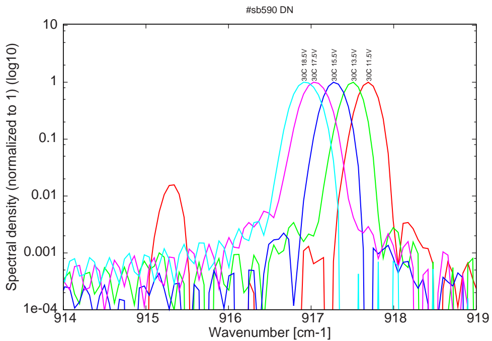
Figure 15: spectra at 30C for various LDD voltages (bimode at threshold)
