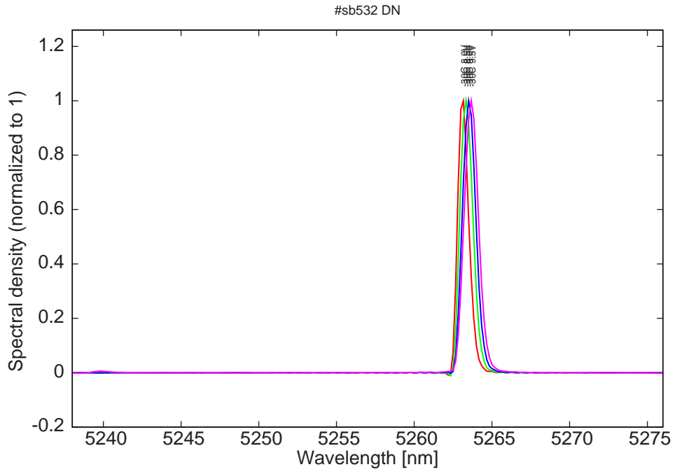
Figure 9: spectra at -30C for various LDD voltages (small mode around 5240 nm)
