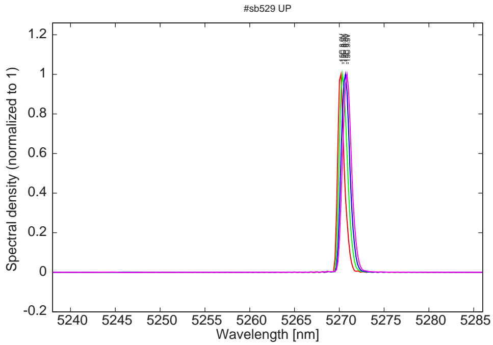
Figure 11: spectra at -15C for various LDD voltages (monomode up to 9V, small mode around 5244 nm)
