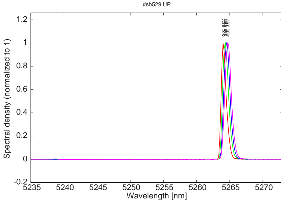
Figure 9: spectra at -30C for various LDD voltages (monomode up to 9V, small mode around 5238 nm)
