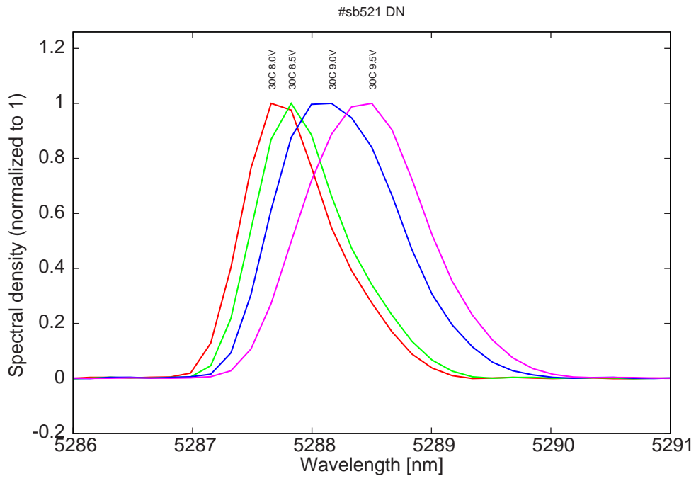
Figure 15: spectra at 30C for various LDD voltages
