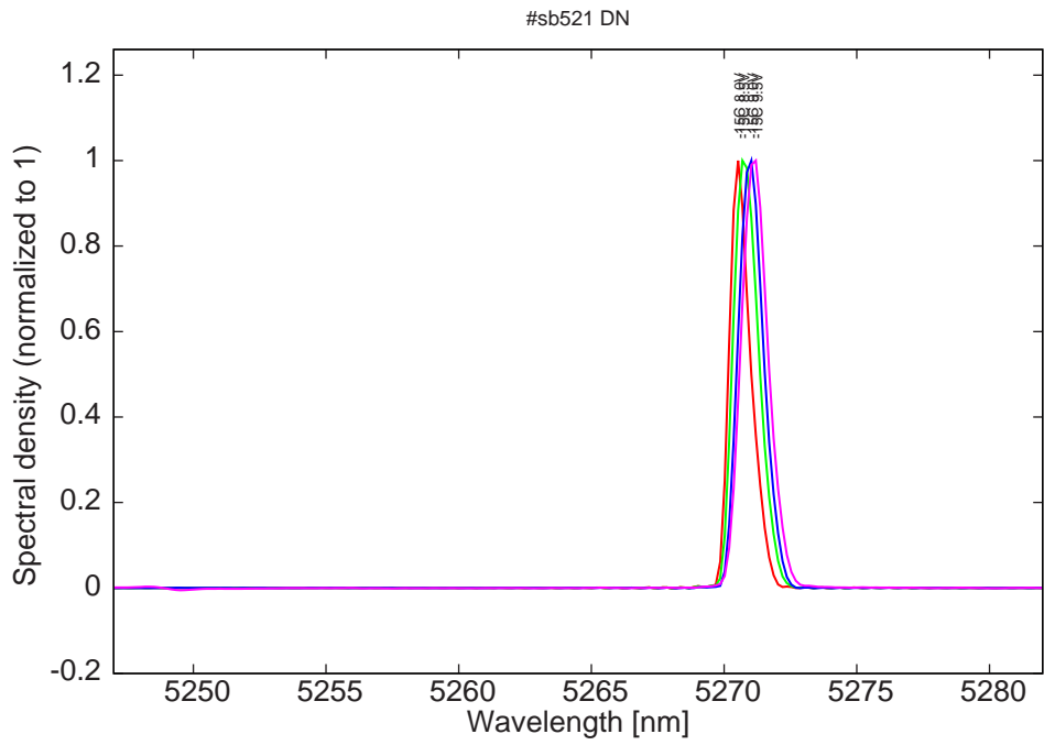
Figure 11: spectra at -15C for various LDD voltages (small mode around 5250 nm)
