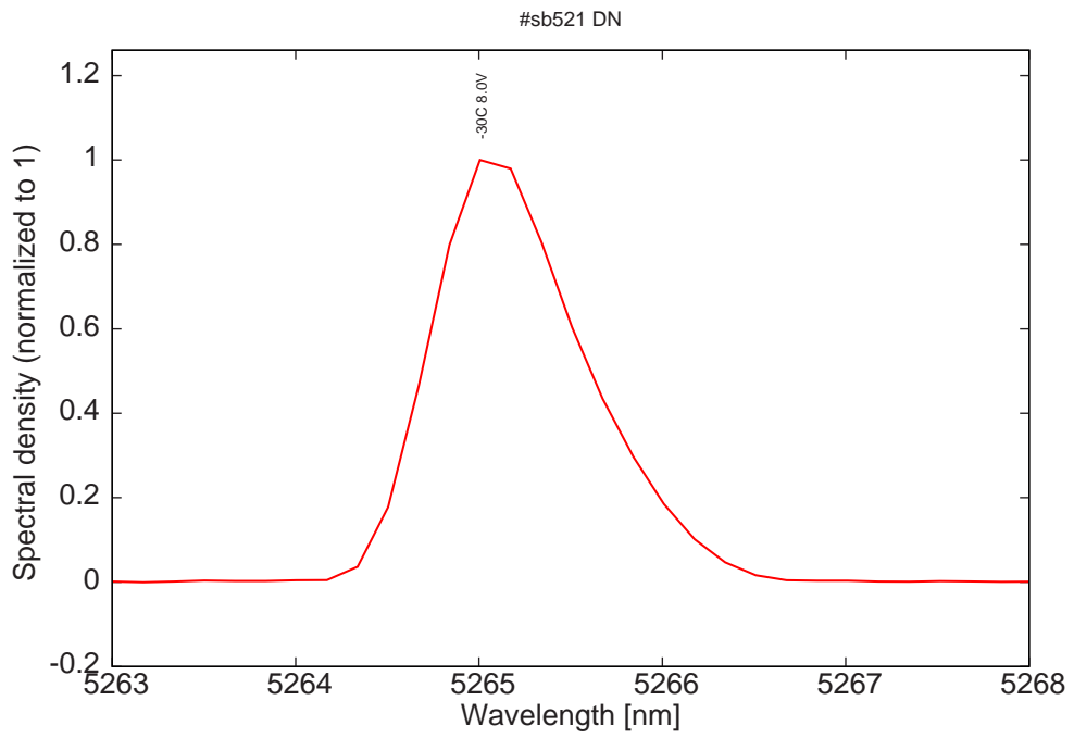
Figure 10: monomode spectrum at -30C and 8V on LDD
