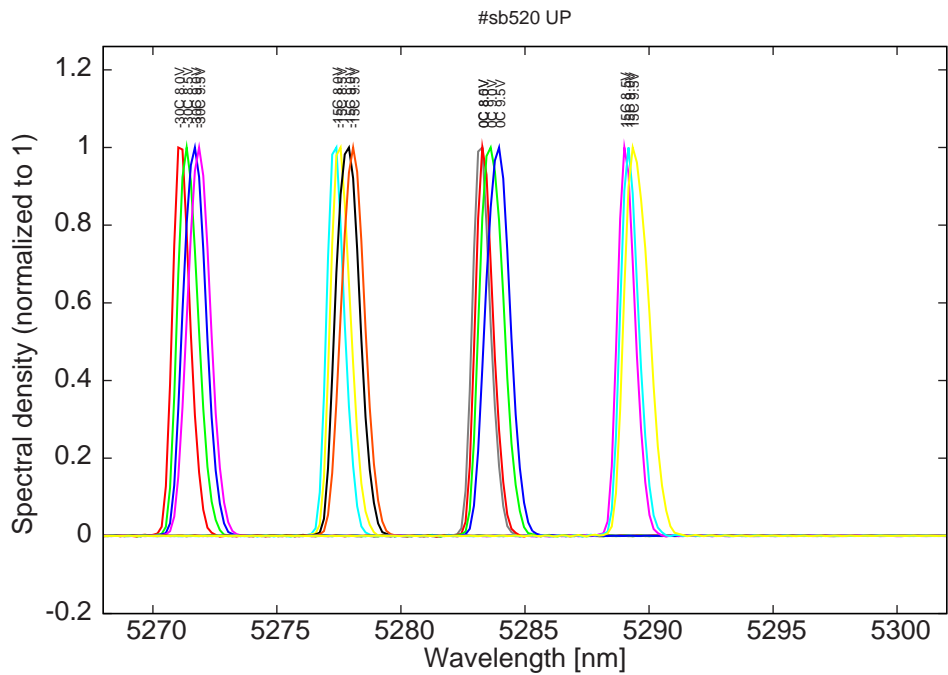
Figure 6: spectra at -30C, -15C, 0C, and 15C at 2% dc for various LDD voltages
