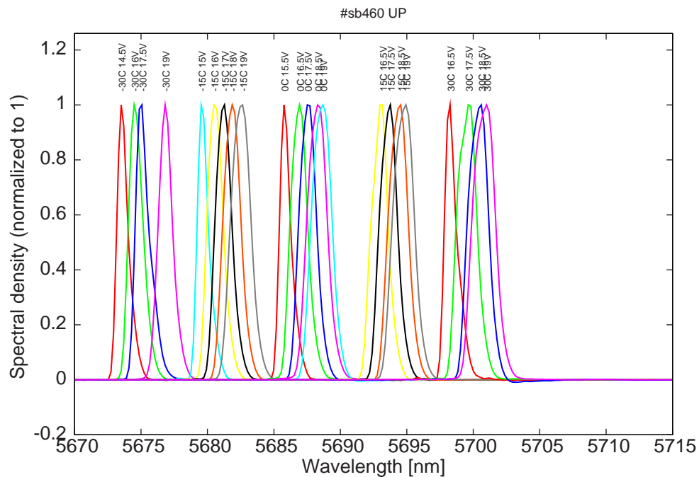
Figure 6: spectra at -30C, -15C, 0C, 15C and 30C at 4% dc for various LDD voltages
