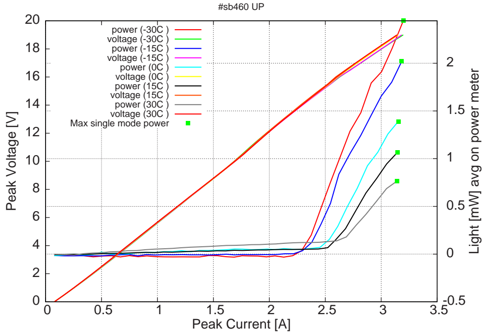
Figure 4: peak voltage and average power vs peak current at 4% dc (the solid squares indicate the maximum singlemode emitted power)
