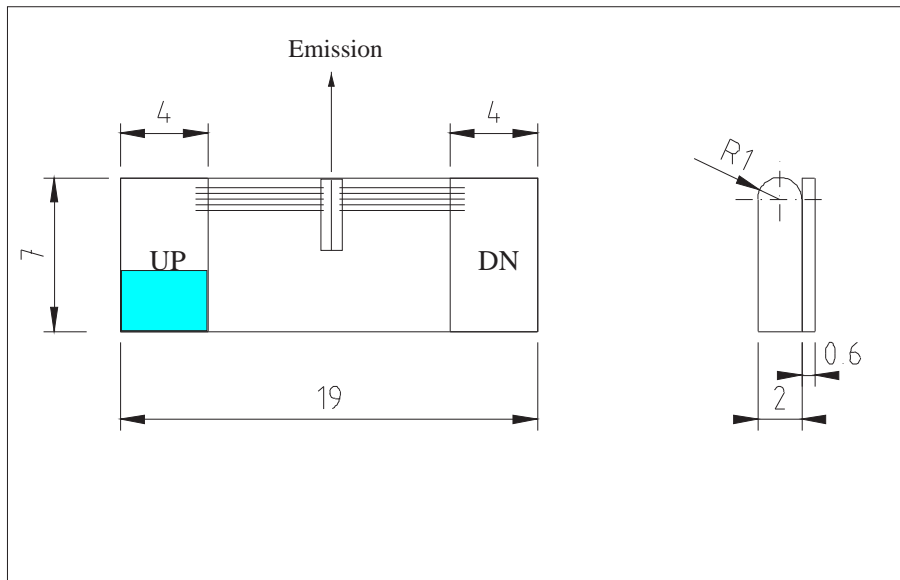
Figure 1: Support mounting for #sb460 UP (please note that the laser is connected to the UP pad drawn in blue)
