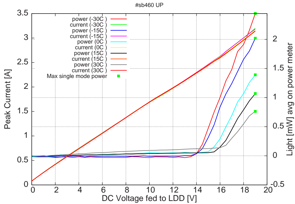
Figure 5: peak current and average power vs LDD voltage at 4% dc (the solid squares indicate the maximum singlemode emitted power)
