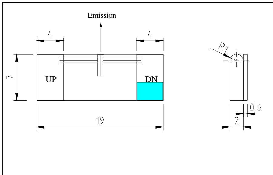
Figure 1: Support mounting for #sb4143 DN (please note that the laser is connected to the DN pad drawn in blue)
