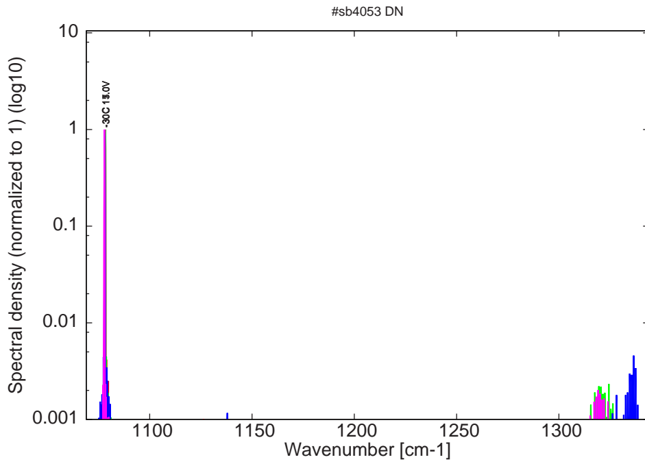
Figure 8: spectra at -30C for various LDD voltages (monomode, then becomes multimode for LDD voltage > 11V)
