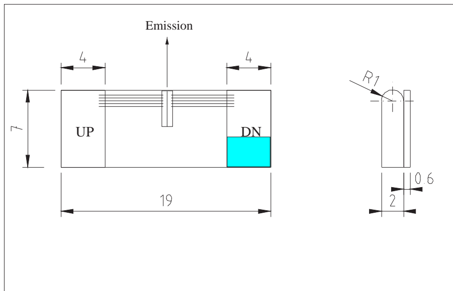
Figure 1: Support mounting for sb4 (please note that the laser is connected to the DN pad drawn in blue)
