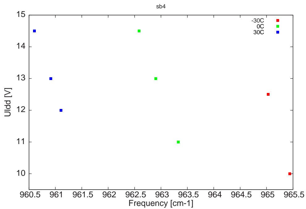
Figure 3: DC voltage fed to LDD ( U_{ddd} ) as a function of the singlemode emission frequencies and temperatures
