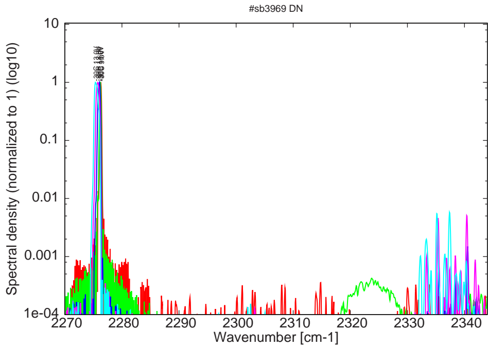
Figure 8: spectra at -30C for various LDD voltages (monomode up to 10V on LDD)
