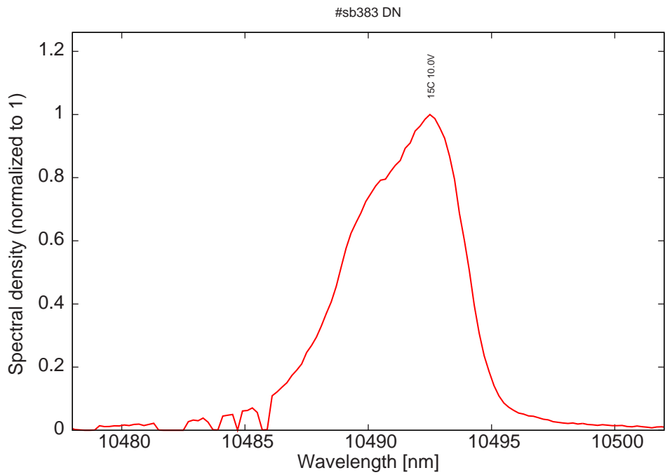
Figure 16: monomode spectrum at 15C at 10.0V on LDD
