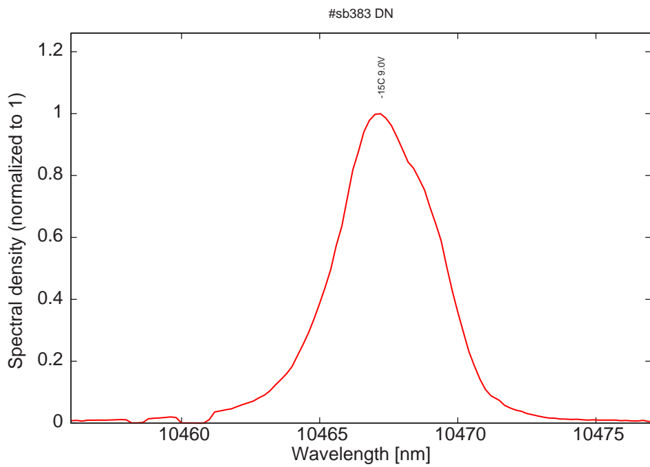
Figure 12: monomode spectrum at -15C at 9.0V on LDD
