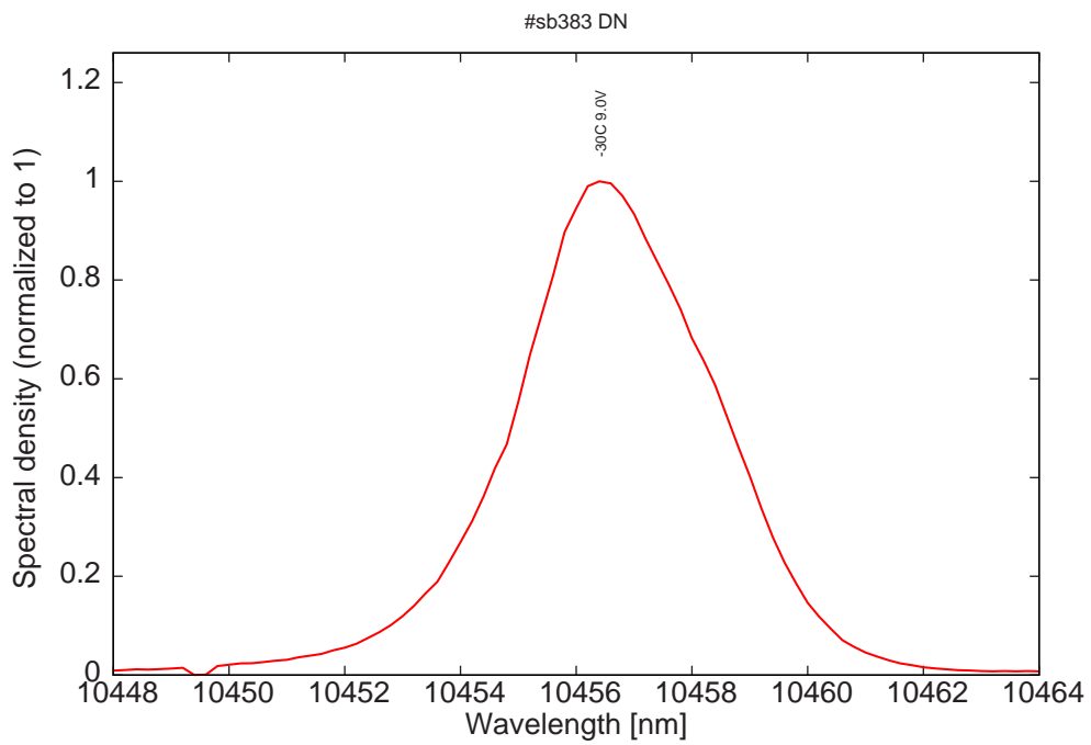
Figure 10: monomode spectrum at -30C at 9.0V on LDD
