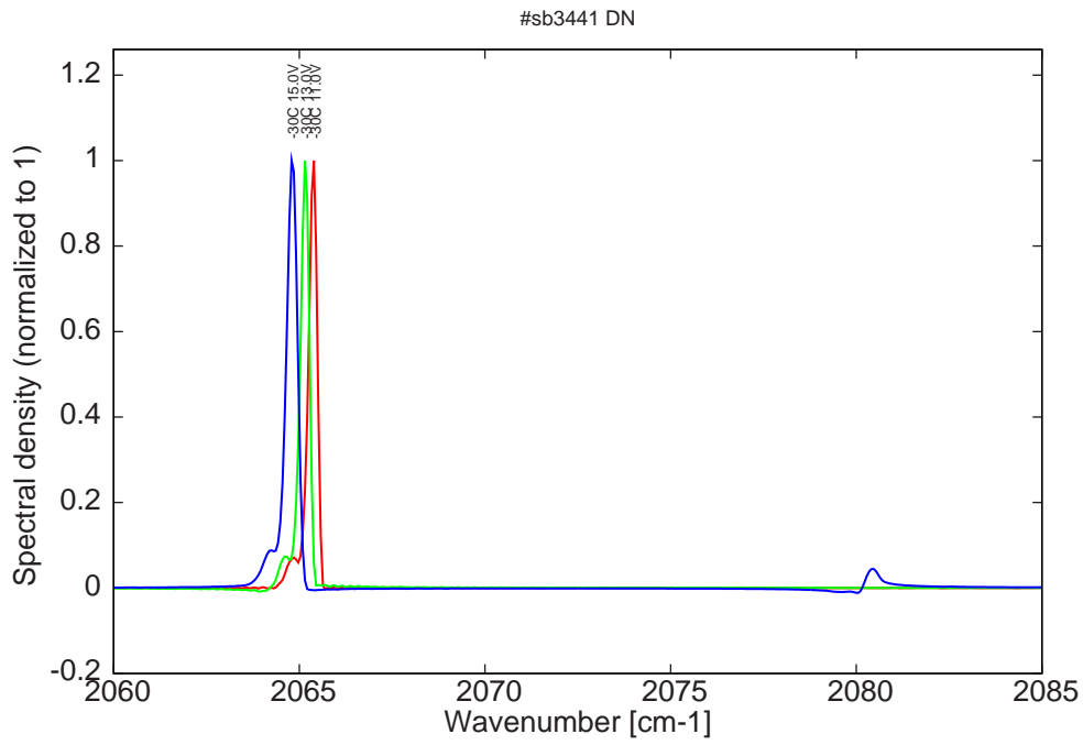
Figure 8: spectra at -30C for various LDD voltages (monomode up to 13V on LDD)
