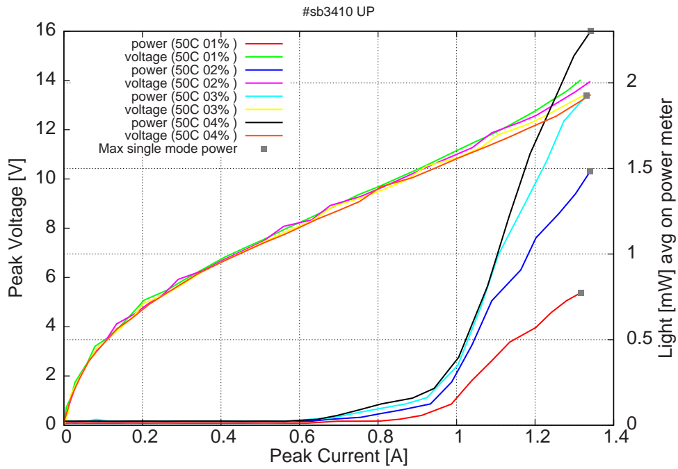
Figure 6: peak voltage and average power vs peak current at 50C for various duty-cycles (100ns pulses on the laser) (the solid squares indicate the maximum singlemode emitted power)
