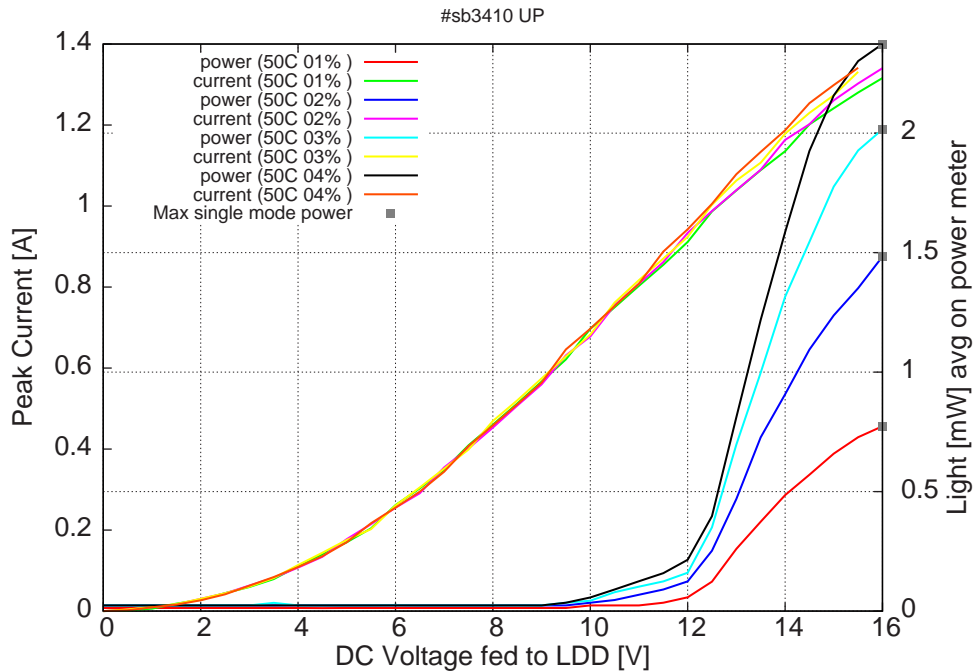
Figure 7: peak current and average power vs LDD voltage at 50C for various duty-cycles (100ns pulses on the laser) (the solid squares indicate the maximum singlemode emitted power)
