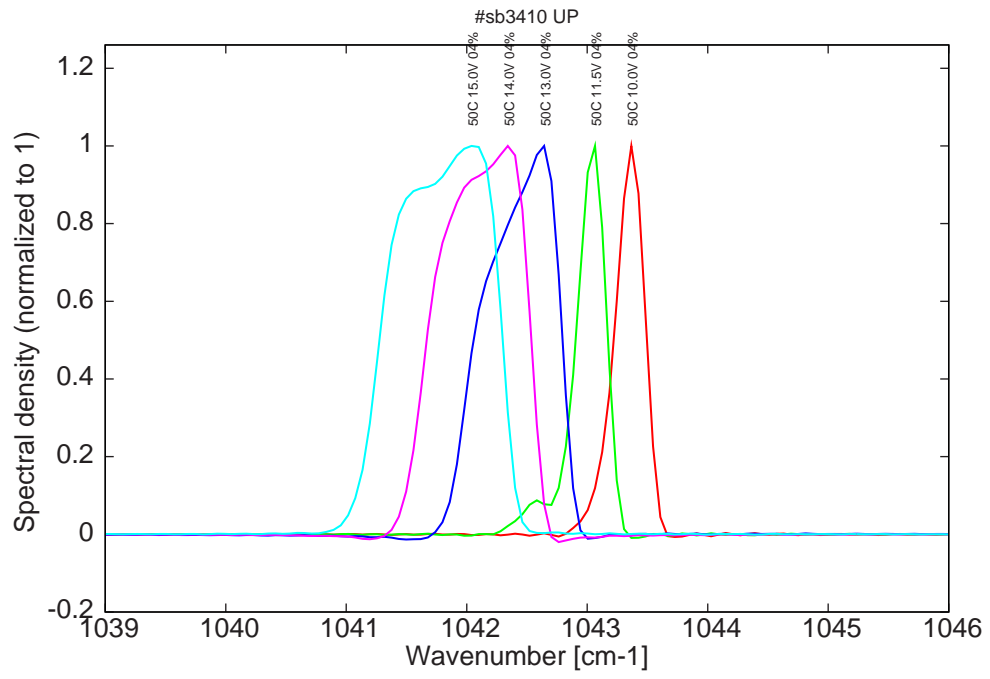
Figure 8: spectra at 50C at 4% duty-cycle for various LDD voltages
