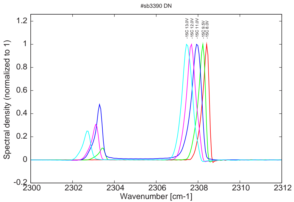
Figure 9: spectra at -15C for various LDD voltages (monomode only at threshold)
