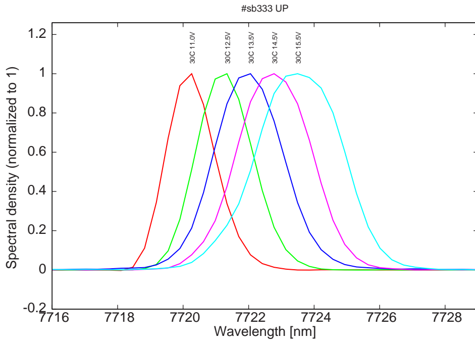
Figure 14: spectra at 30C for various LDD voltages
