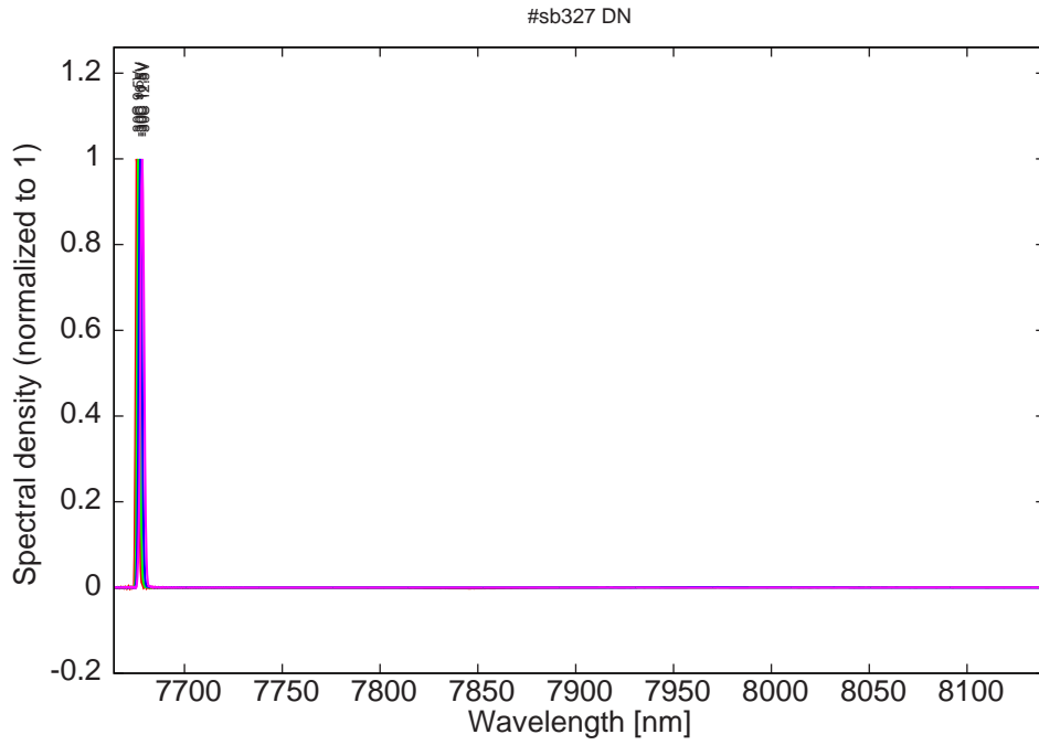
Figure 9: spectra at -30C for various LDD voltages (small modes around 8050 nm for 12.5V on LDD)
