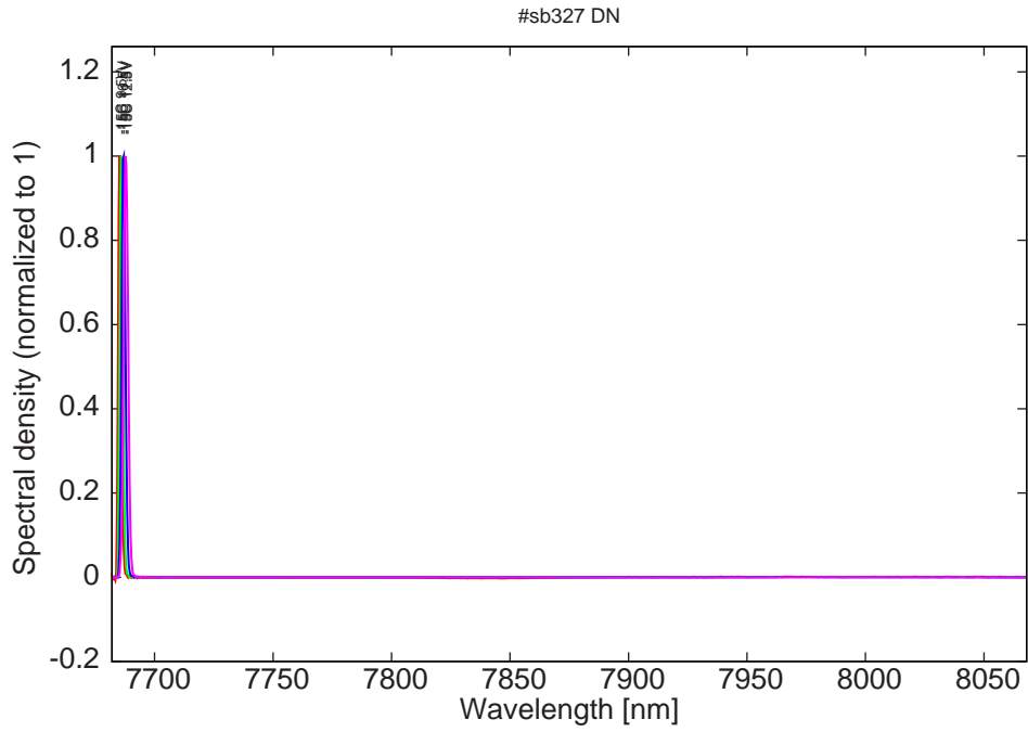
Figure 11: spectra at -15C for various LDD voltages (small modes around 8050 nm for 12.5V on LDD)
