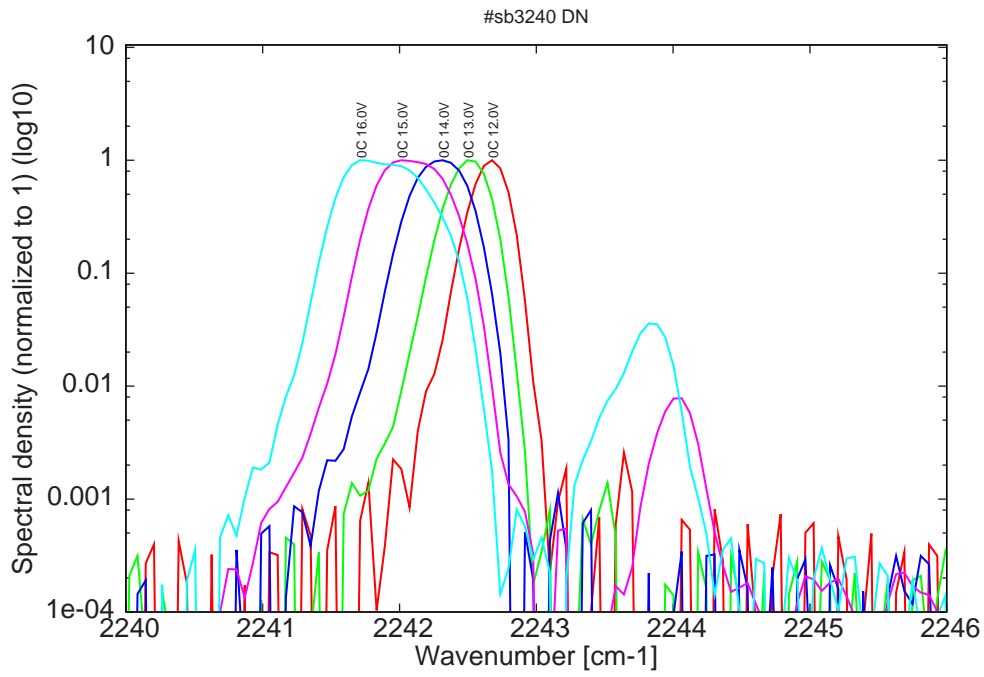
Figure 10: spectra at 0C for various LDD voltage (monomode up to 14.0V on LDD)
