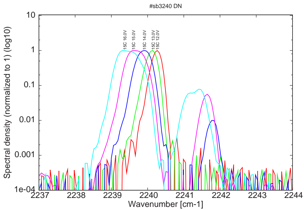
Figure 11: spectra at 15C for various LDD voltage (monomode up to 13.0V on LDD)
