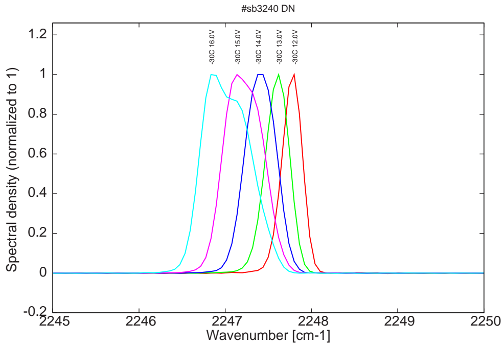
Figure 8: spectra at -30C for various LDD voltage (all monomode)
