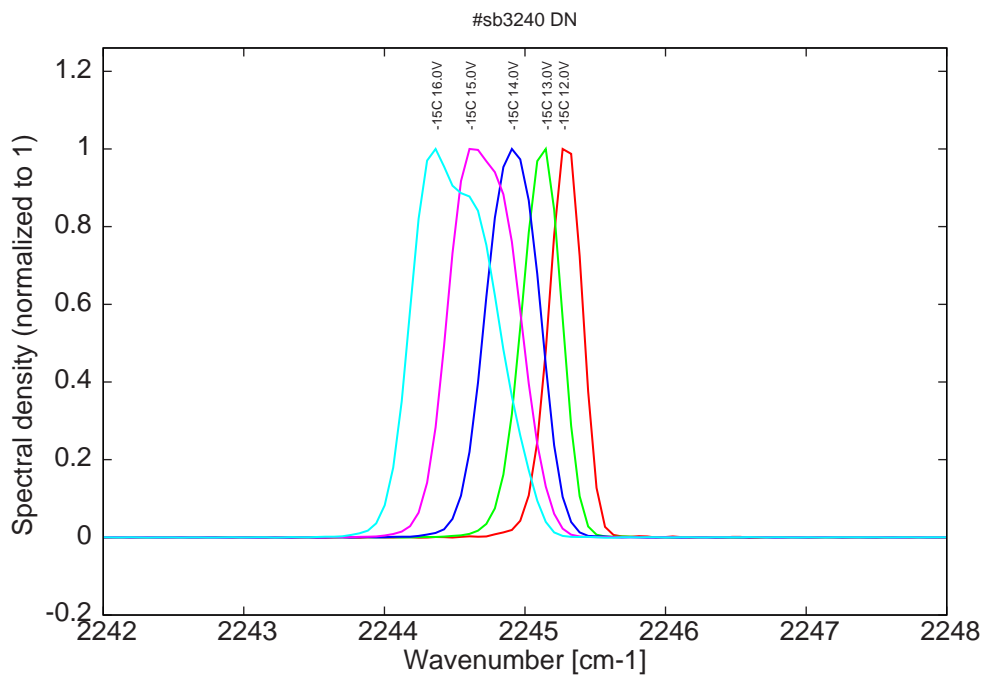
Figure 9: spectra at -15C for various LDD voltage (all monomode)
