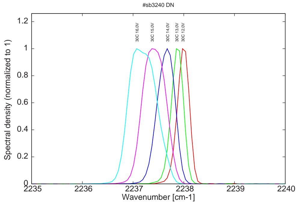
Figure 12: spectra at 30C for various LDD voltage (all monomode)
