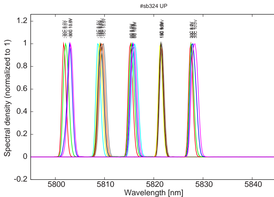
Figure 6: spectra at -30C, -15C, 0C, 15C and 30C at 2%dc for various LDD voltage
