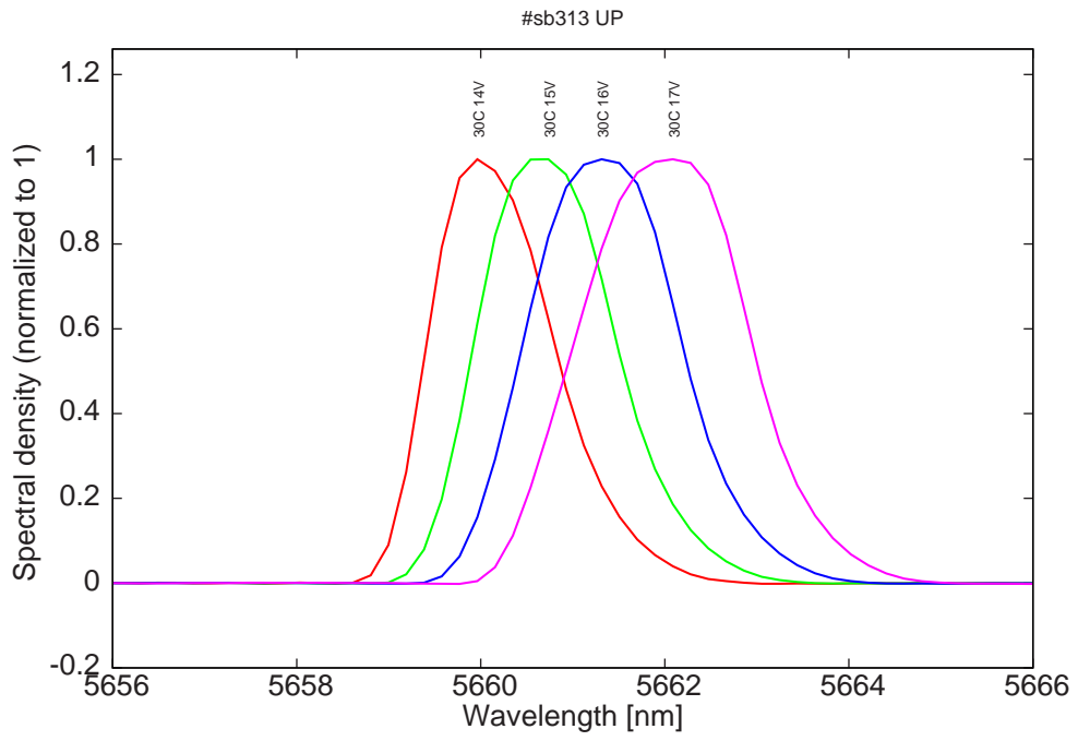
Figure 15: spectra at 30C for various LDD voltage (all monomode)
