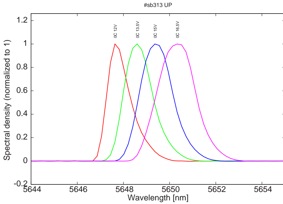
Figure 13: spectra at 0C for various LDD voltage (all monomode)
