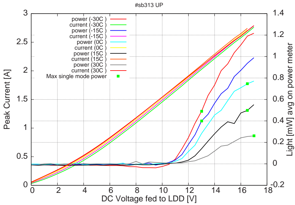
Figure 7: peak current and average power vs LDD voltage at 4%dc (including the multi-mode region)
