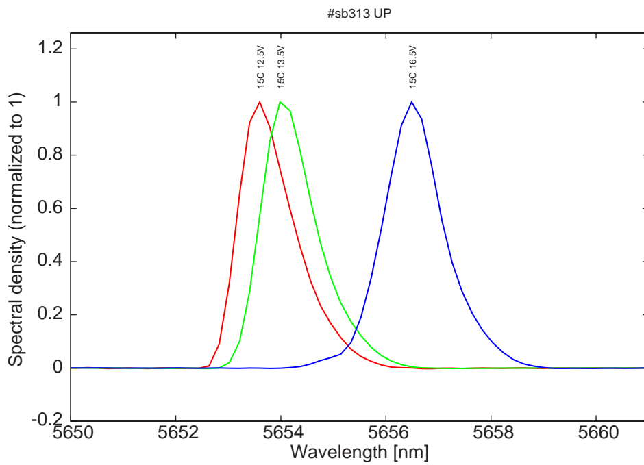
Figure 14: spectra at 15C for various LDD voltage (all monomode)
