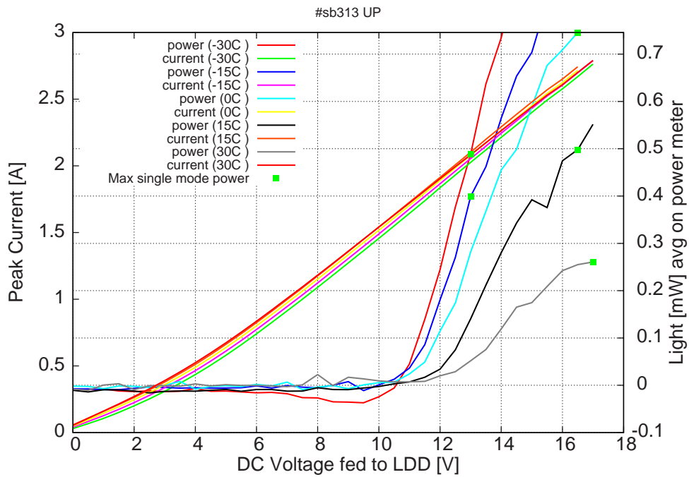
Figure 6: peak current and average power vs LDD voltage at 4%dc (the solid squares indicate the maximum singlemode emitted power)
