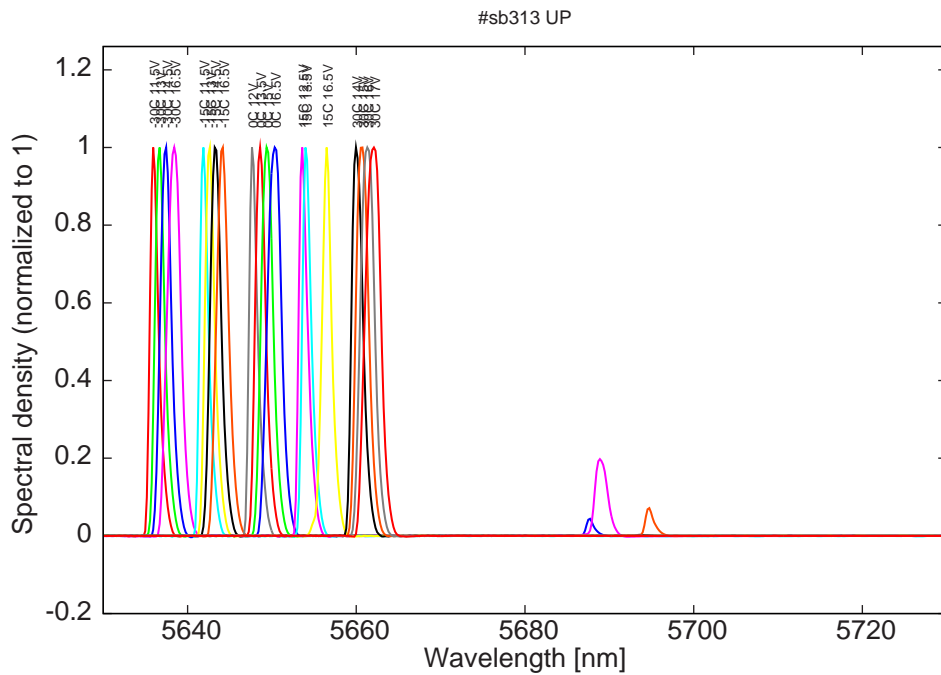
Figure 8: spectra at -30C, -15C, 0C, 15C and 30C at 4%dc for various LDD voltage
