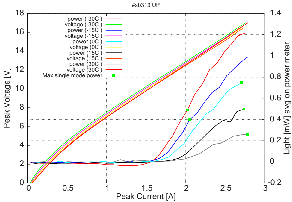
Figure 5: peak voltage and average power vs peak current at 4%dc (including the multi-mode region)
