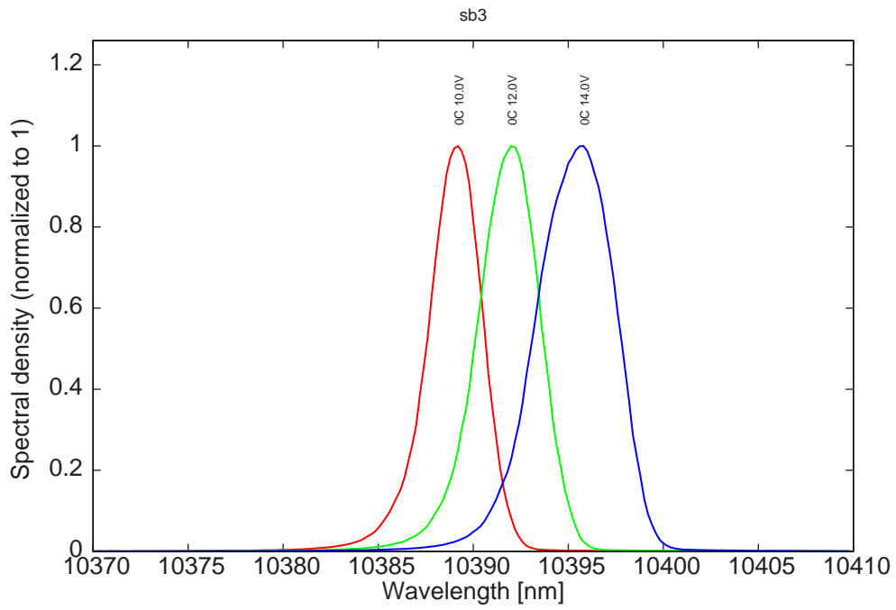
Figure 7: spectra at 0°C for various LDD voltages
