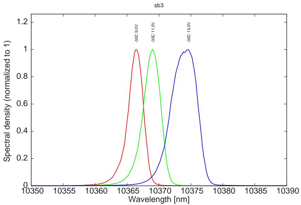
Figure 6: spectra at -30^{\circ}\text{C} for various LDD voltages
