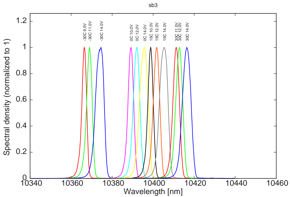
Figure 10: spectra (overview from -30^{\circ}\text{C} to 30^{\circ}\text{C} ) for various LDD voltages
