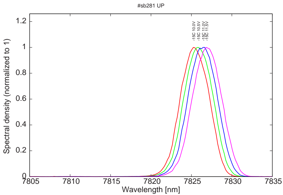
Figure 10: spectra at -15C for various LDD voltages (mode around 7810nm)
