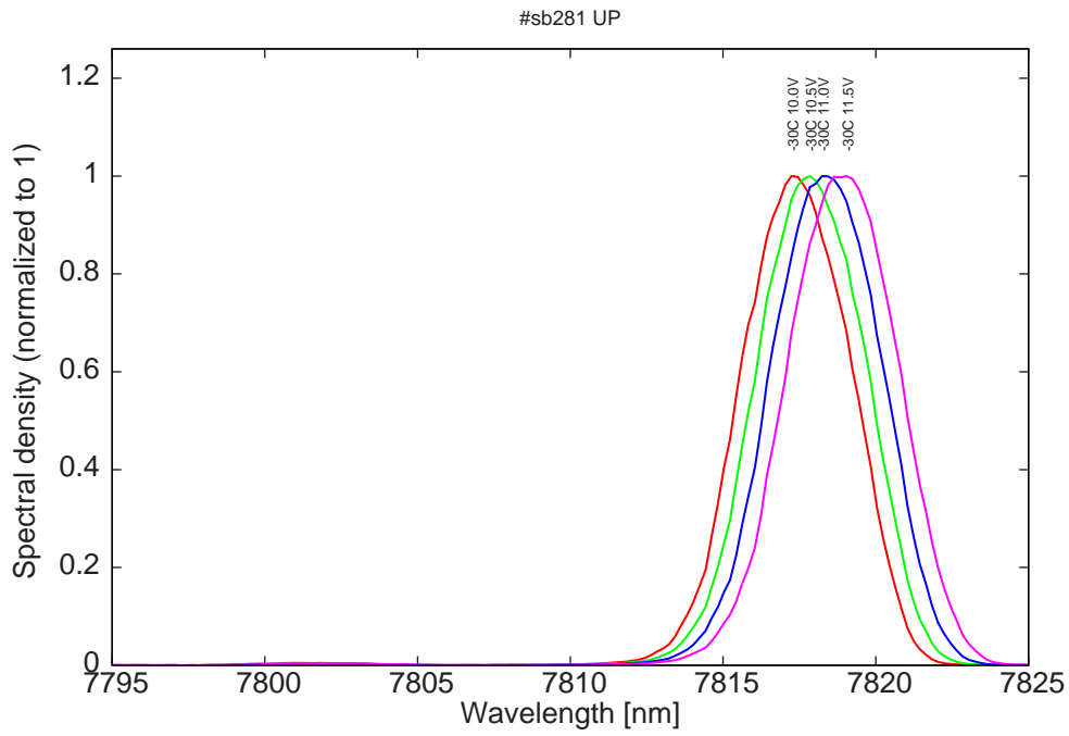
Figure 9: spectra at -30C for various LDD voltages (all bimodes: mode around 7802nm)
