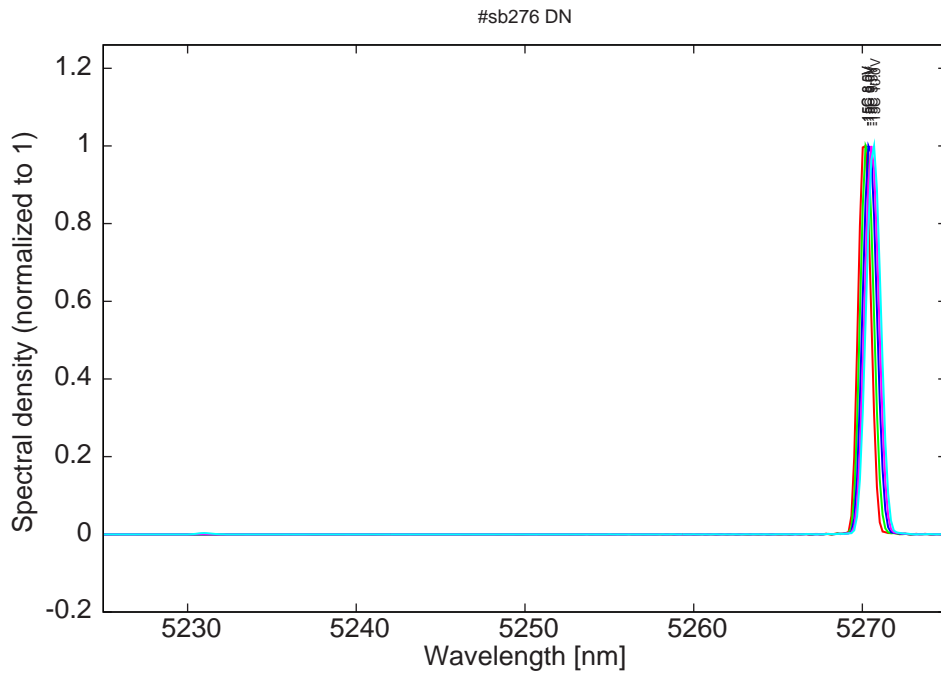
Figure 11: spectra at -15C for various LDD voltages (modes around 5231 nm)
