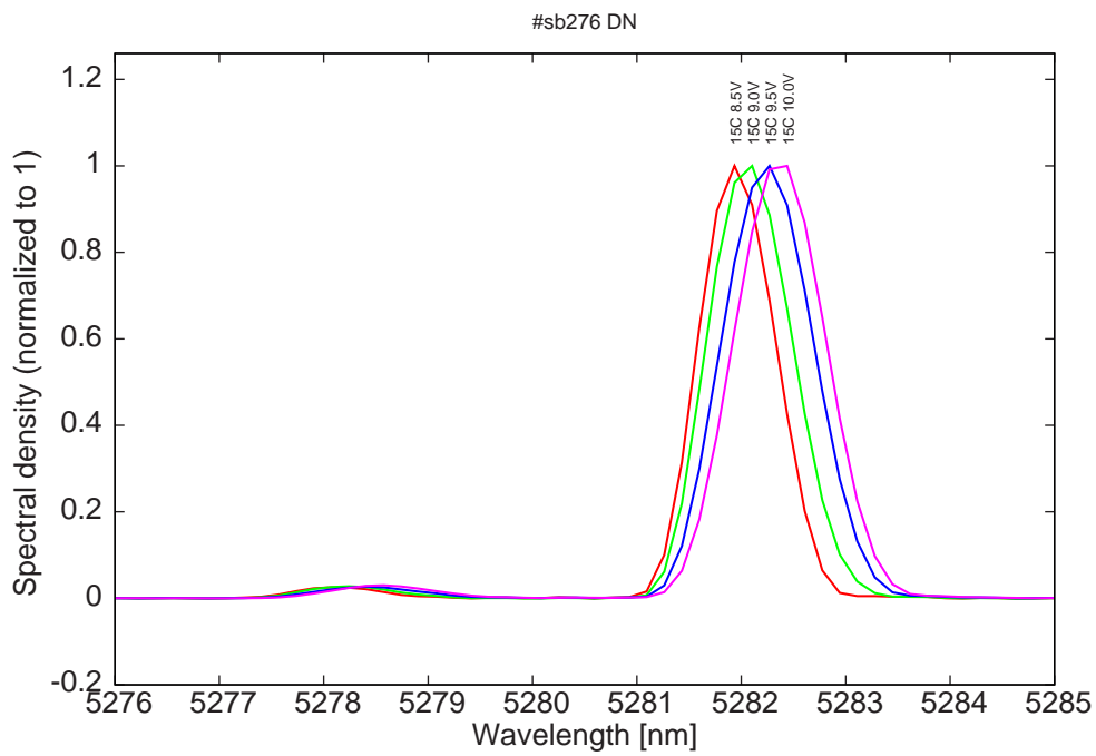
Figure 14: spectra at 15C for various LDD voltages (all biomodes)
