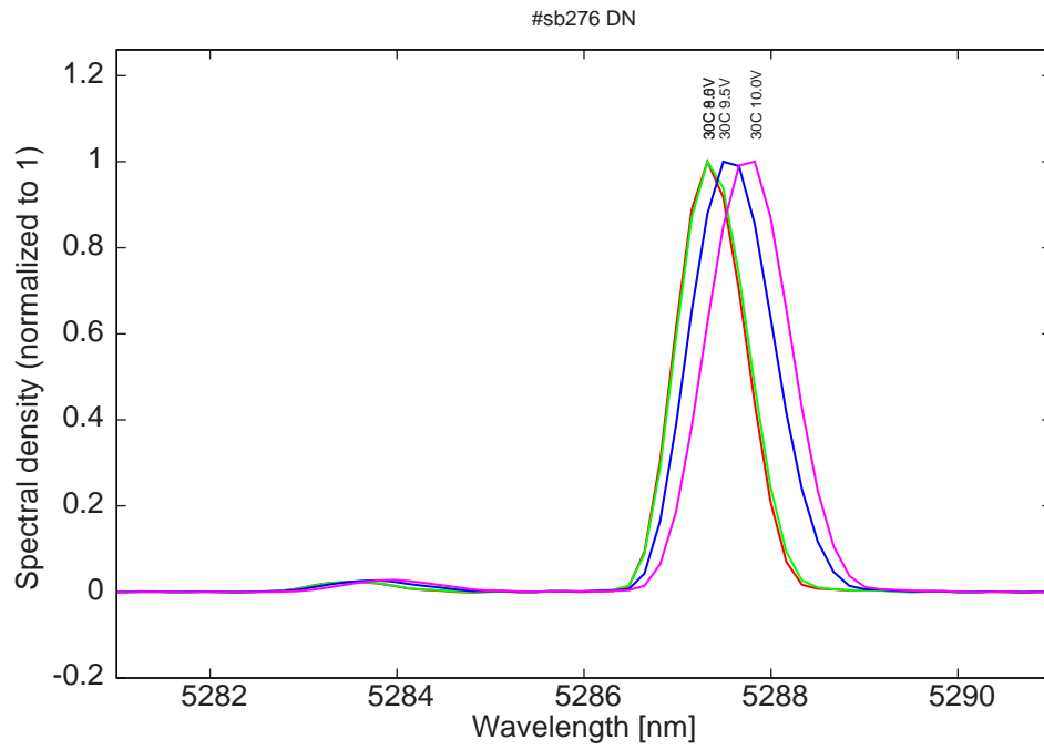
Figure 15: spectra at 30C for various LDD voltages (all bimodes)
