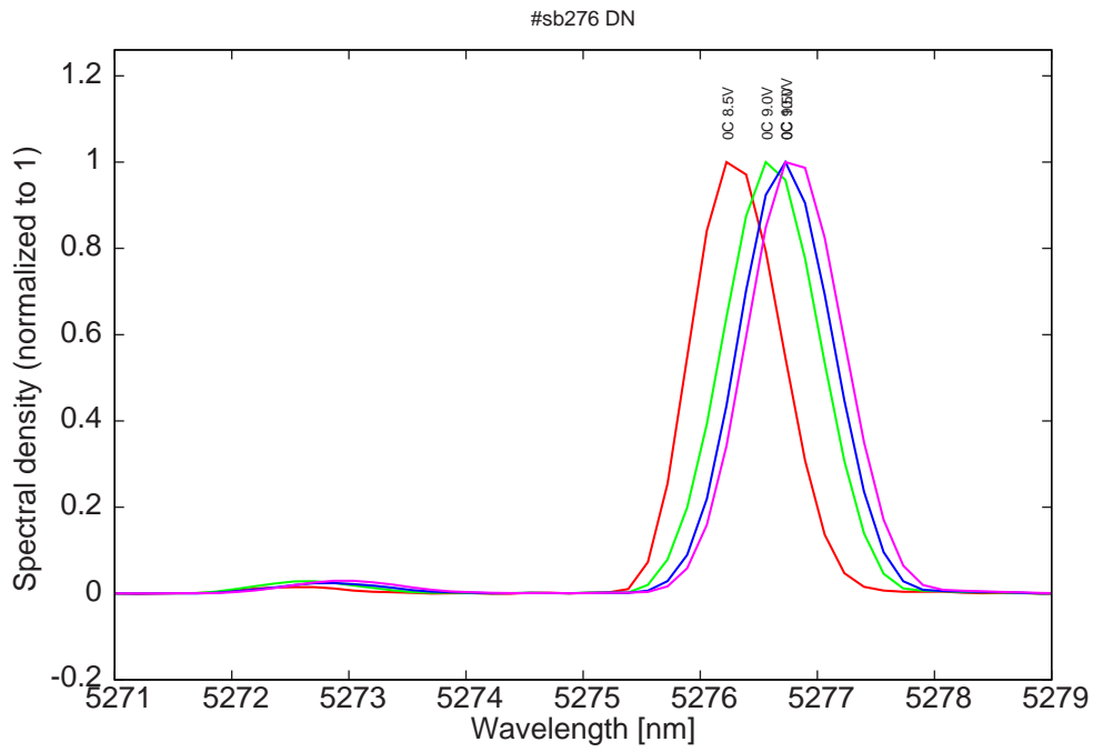
Figure 13: spectra at 0C for various LDD voltages (all bimodes)
