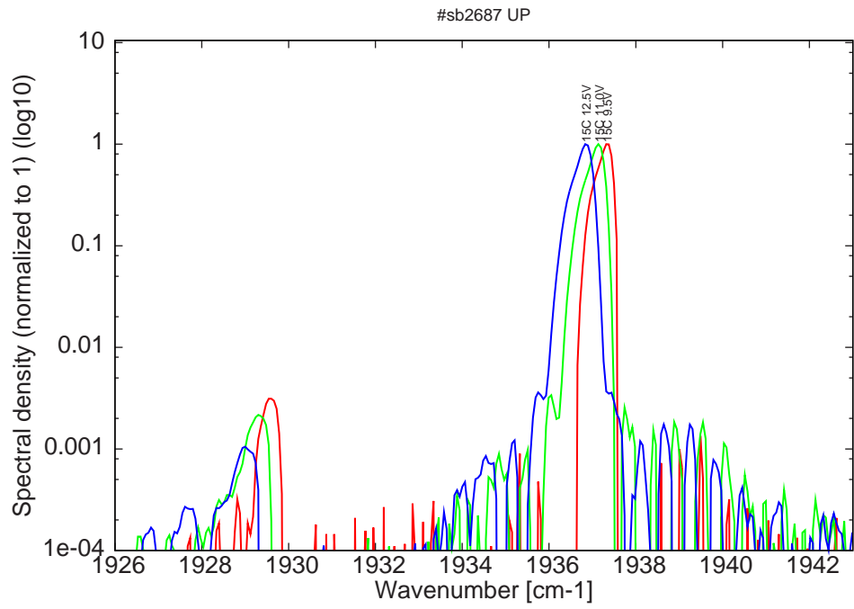
Figure 10: spectra 15C for various LDD voltages at 2% duty cycle (22ns pulses on the laser), all bimode
