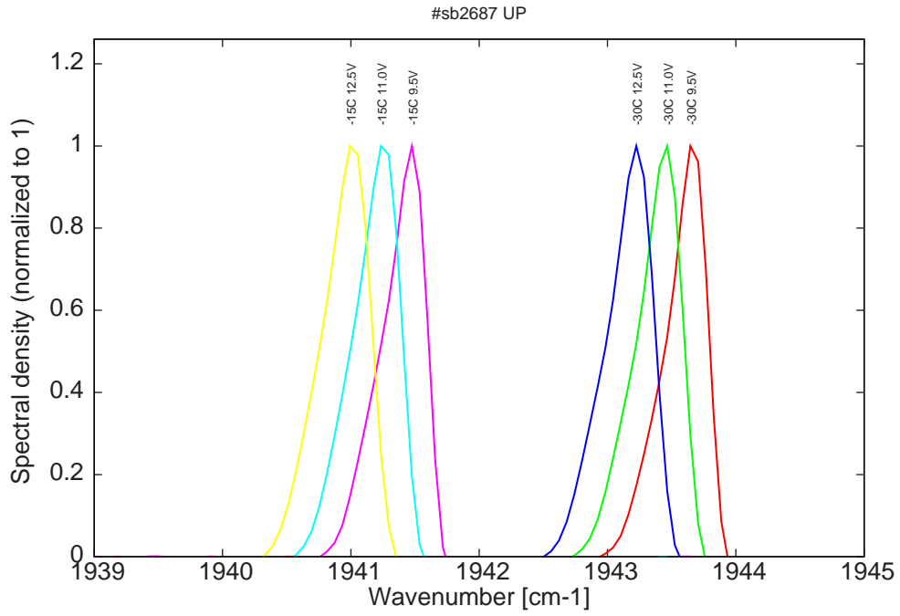
Figure 8: spectra at -30C and -15C for various LDD voltages at 2% duty cycle (22ns pulses on the laser), all monomode
