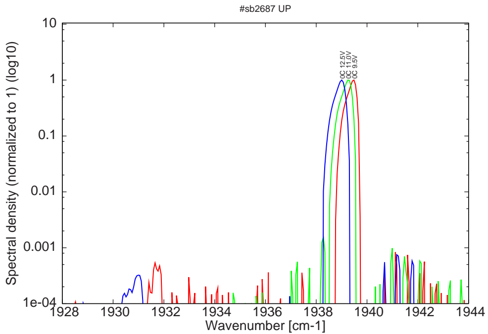
Figure 9: spectra 0C for various LDD voltages at 2% duty cycle (22ns pulses on the laser), monomode only at threshold, small mode around 1931cm-1
