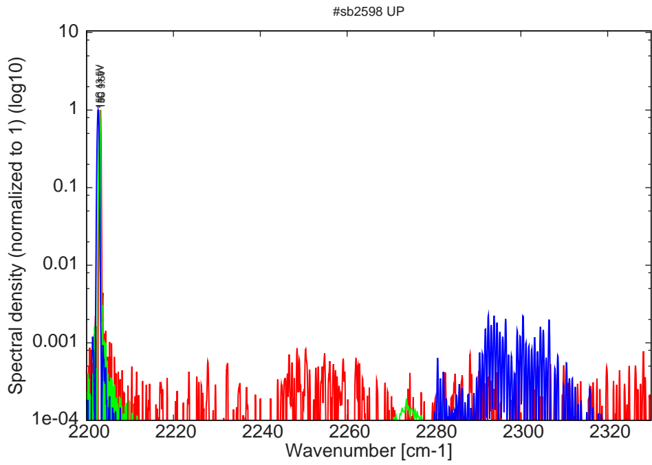
Figure 14: spectra at ^{15}\text{C} at various LDD voltages at 2% duty-cycle (22ns pulses on the laser)
