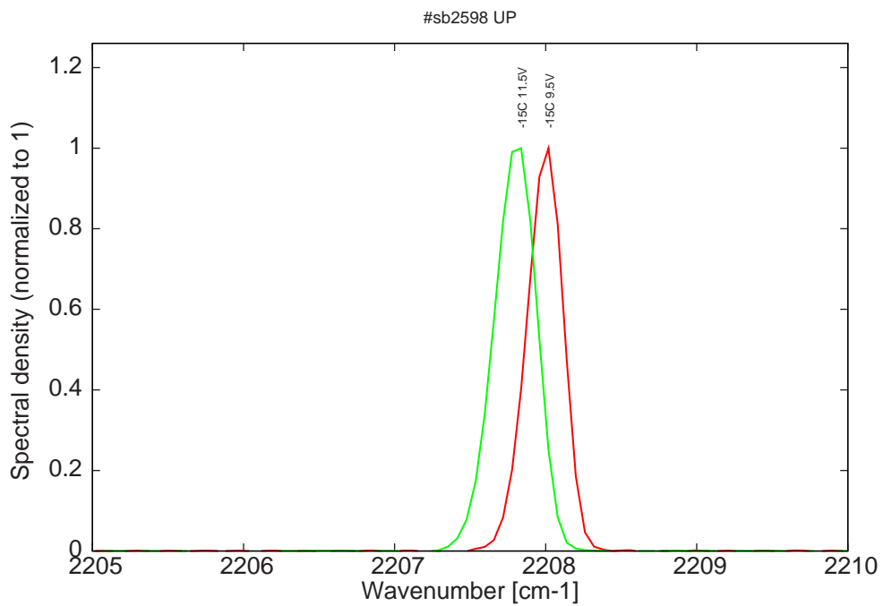
Figure 11: spectra at -15C at various LDD voltages at 2% duty-cycle (monomode range)
