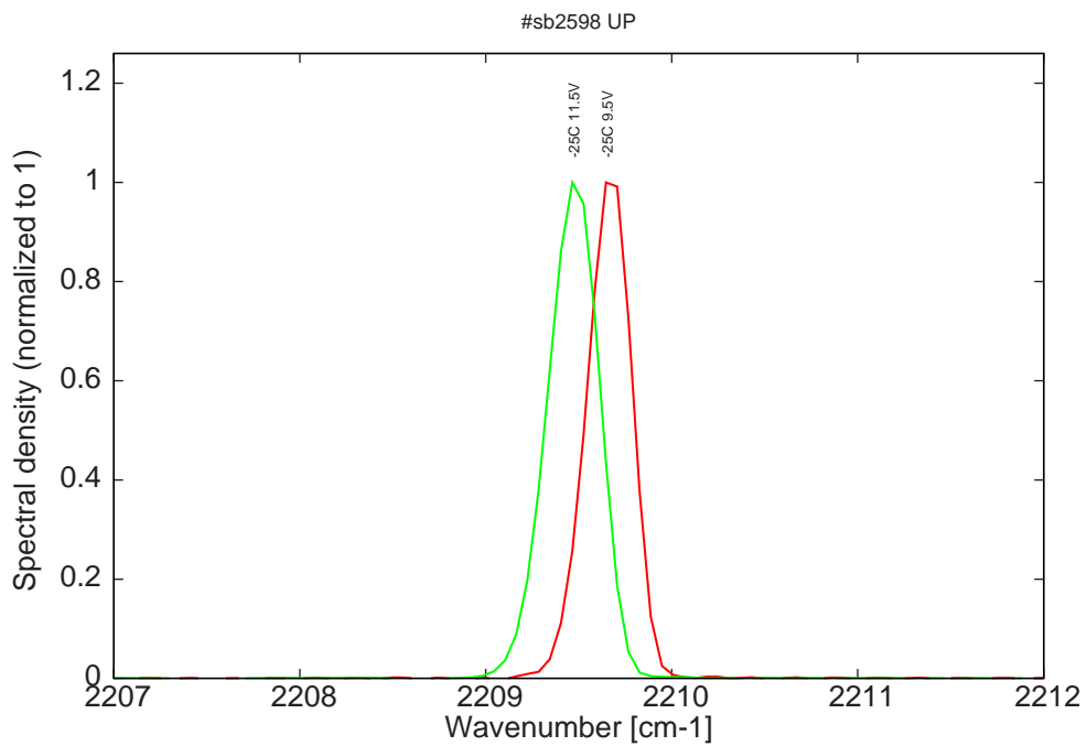
Figure 9: spectra at -25C at various LDD voltages at 2% duty-cycle (monomode range)
