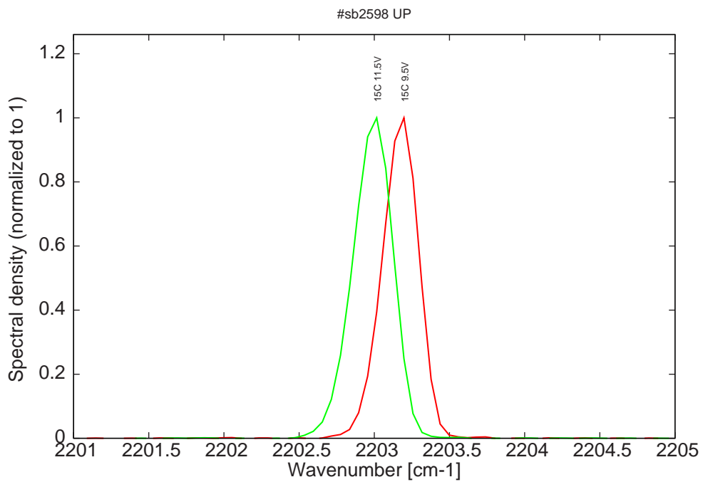
Figure 15: spectra at ^{15}\text{C} at various LDD voltages at 2% duty-cycle (monomode range)
