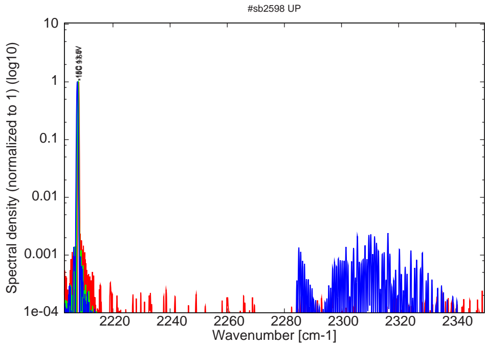
Figure 10: spectra at -15C at various LDD voltages at 2% duty-cycle (22ns pulses on the laser)
