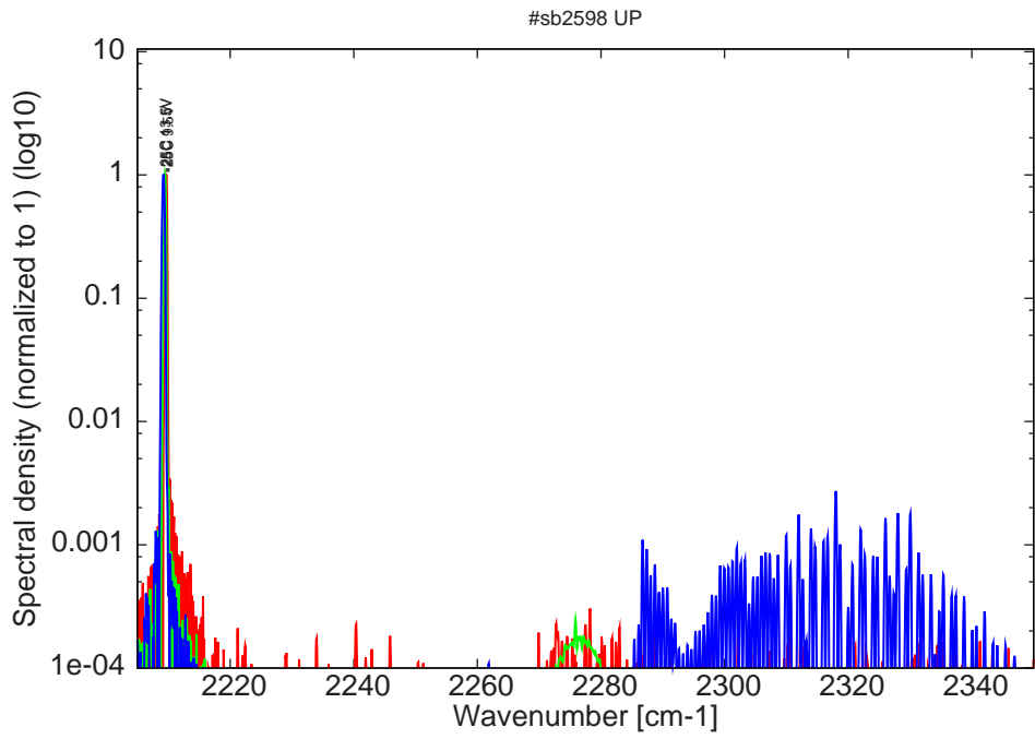
Figure 8: spectra at -25C at various LDD voltages at 2% duty-cycle (22ns pulses on the laser)
