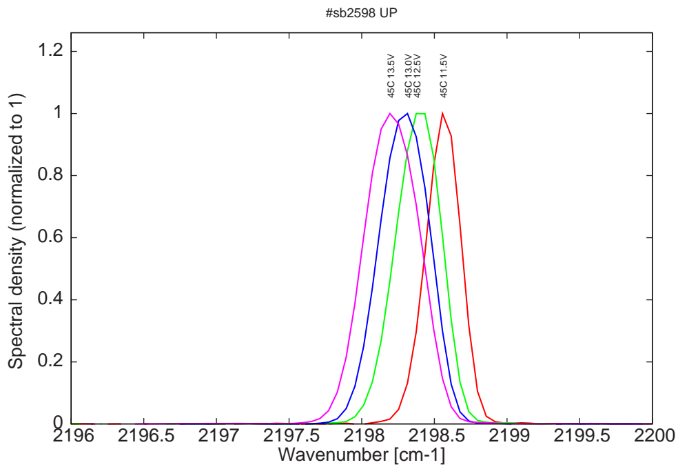
Figure 19: spectra at 45C at various LDD voltages at 2% duty-cycle (monomode range)
