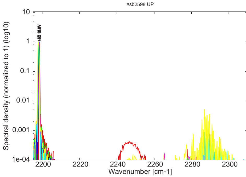
Figure 18: spectra at 45C at various LDD voltages at 2% duty-cycle (22ns pulses on the laser)
