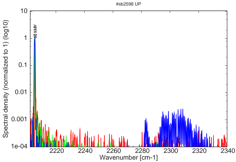
Figure 12: spectra at 0C at various LDD voltages at 2% duty-cycle (22ns pulses on the laser)
