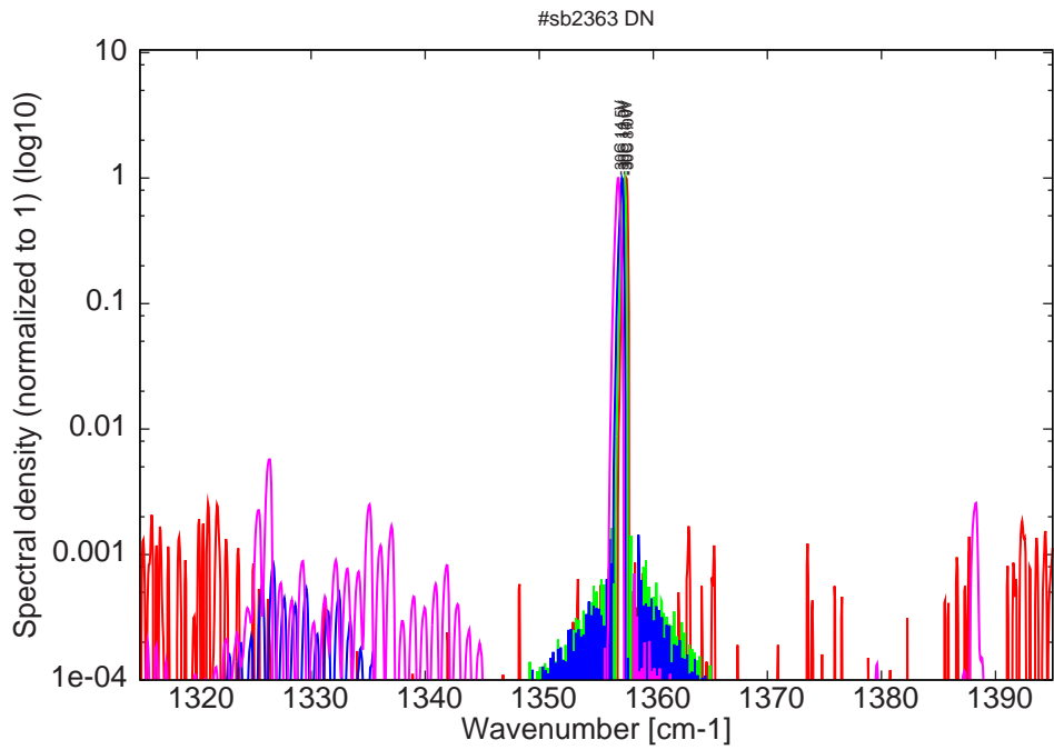
Figure 8: spectra at -30C for various LDD voltages (22ns pulses, 1.1\mu\text{s} period) (monomode up to 10V)
