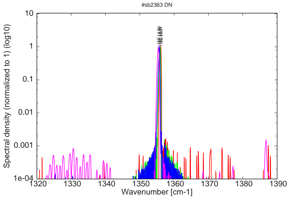
Figure 10: spectra at -15C for various LDD voltages (22ns pulses, 1.1 \mu s period) (monomode up to 12V)
