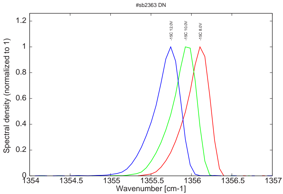
Figure 11: spectra at -15C for various LDD voltages (22ns pulses, 1.1 \mu s period) (monomode range)
