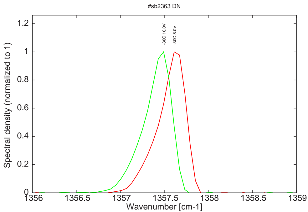
Figure 9: spectra at -30C for various LDD voltages (22ns pulses, 1.1\mu\text{s} period) (monomode range)
