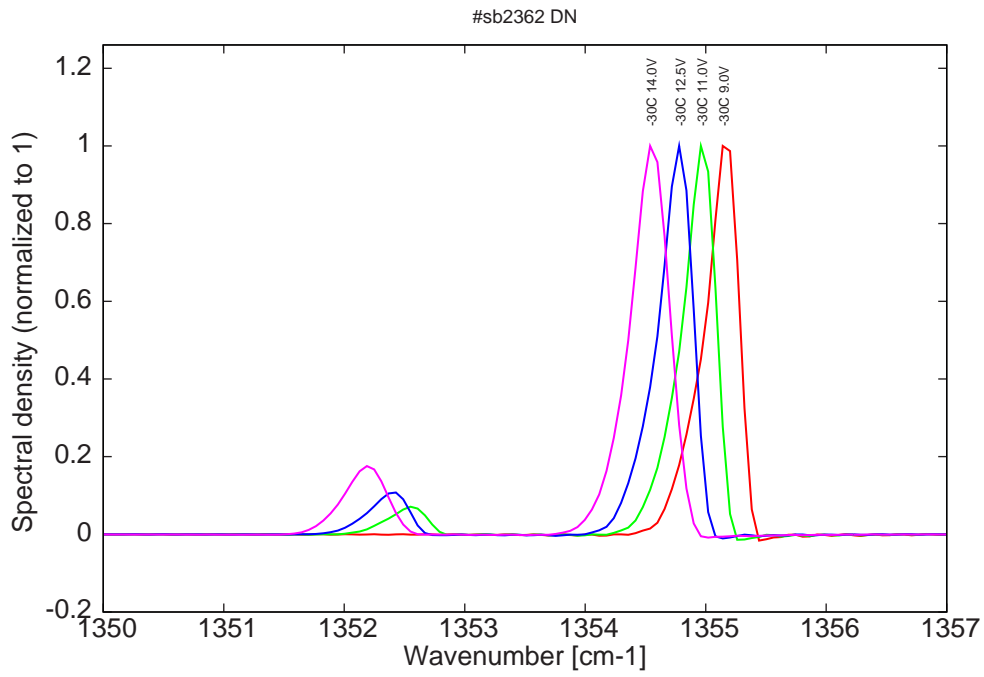
Figure 8: spectra at -30C for various LDD voltages (22ns pulses, 1.1 \mu s period) (monomode only at threshold)
