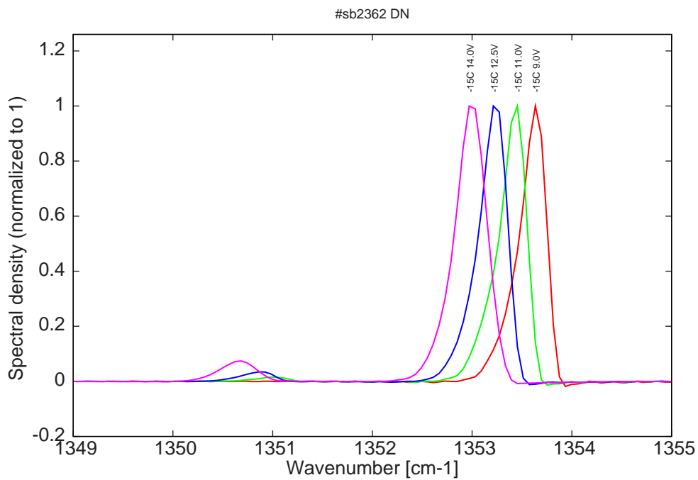
Figure 9: spectra at -15C for various LDD voltages (22ns pulses, 1.1 \mu s period) (monomode only at threshold)
