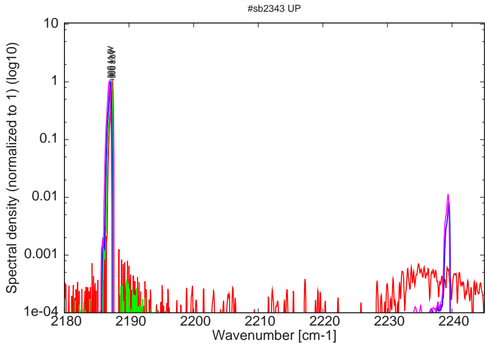
Figure 8: spectra at -30C for various LDD voltages, monomode up to 9.5V (22ns pulses, 1.1us period)
