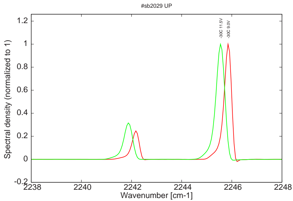
Figure 8: spectra at -30C for various LDD voltage (22ns pulses on the laser); all bimode
