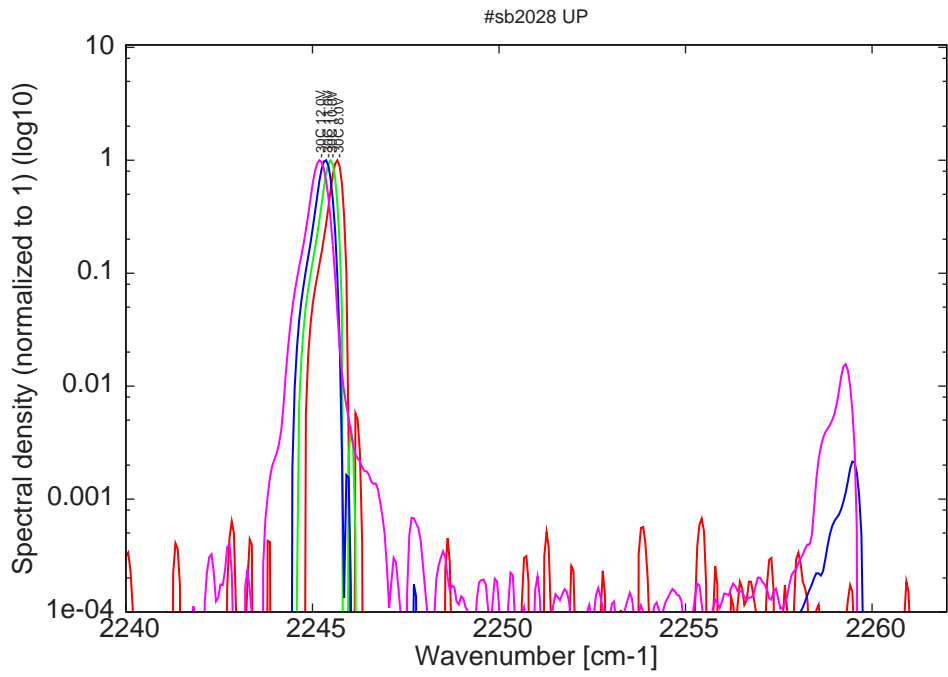
Figure 8: spectra at -30C for various LDD voltage (22ns pulses on the laser)
