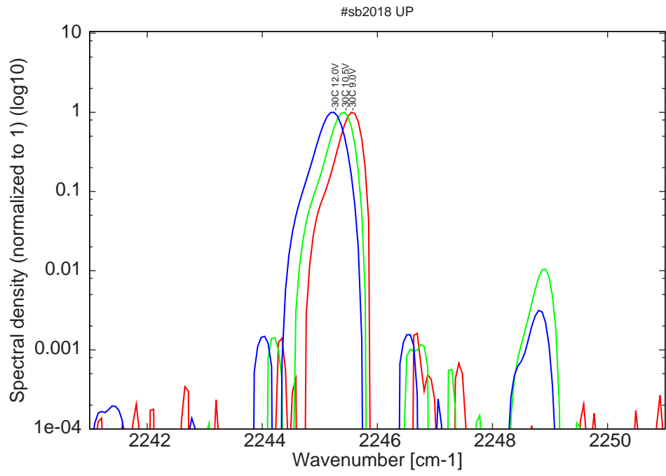
Figure 8: spectra at -30C for various LDD voltage (22ns pulses on the laser); monomode only at threshold
